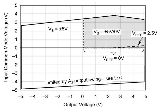
Figure 6-3. Input Common-Mode Range vs Output Voltage, V_S = \pm 5V , G = 5
