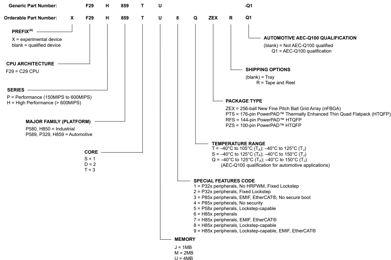
Figure 9-1. Device Nomenclature
