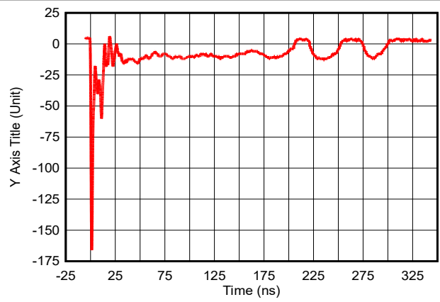
Figure 5-12. -8kV Clamped IEC Waveform (DPY)
