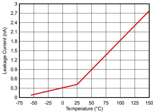
Figure 5-15. Temperature vs. Leakage Current (DPY)
