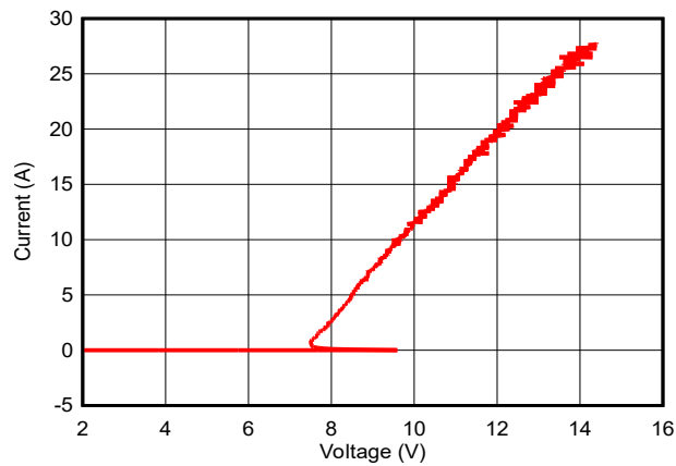
Figure 5-9. Positive TLP Curve (DPY)
