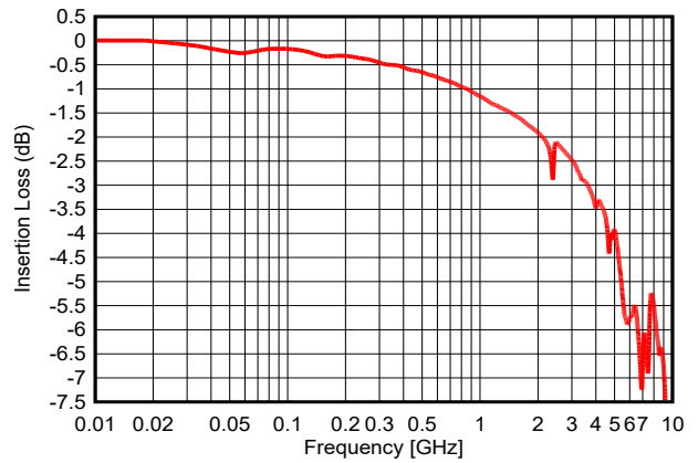
Figure 5-16. Insertion Loss (DPY)
