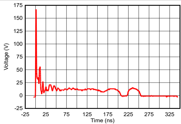
Figure 5-11. +8kV Clamped IEC Waveform (DPY)
