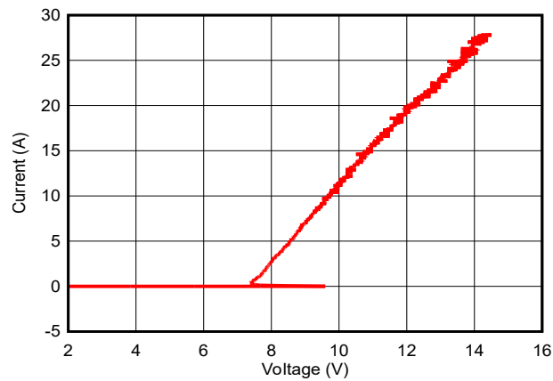
Figure 5-10. Negative TLP Curve (DPY)
