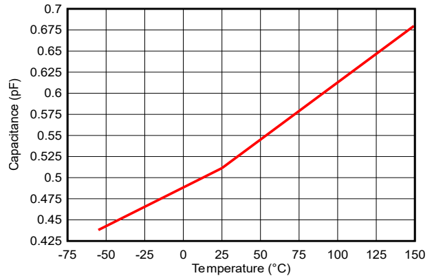
Figure 5-14. Temperature vs. Capacitance (DPY)
