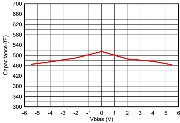
Figure 5-13. Bias Voltage vs. Capacitance (DPY)
