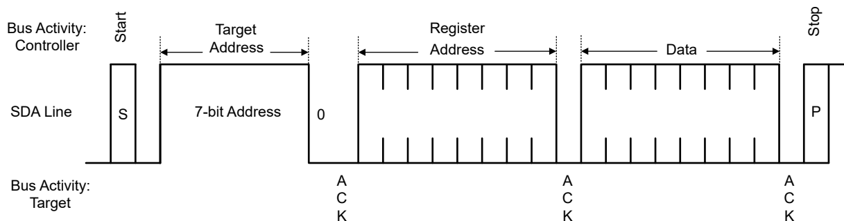
Figure 5-24. Serial Control Bus — WRITE
