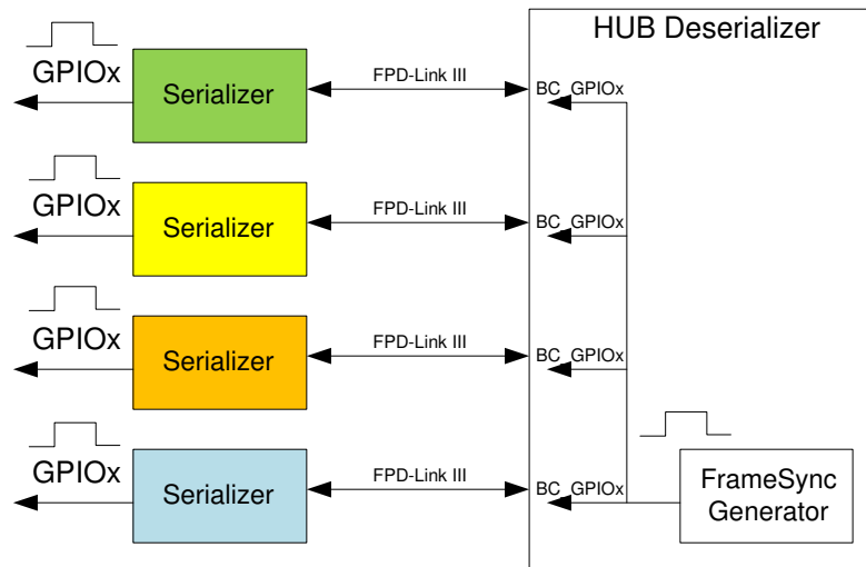
Figure 5-16. Internal FrameSync
