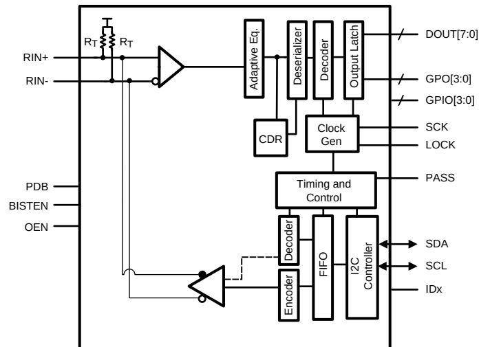
Figure 2. Block Diagram
