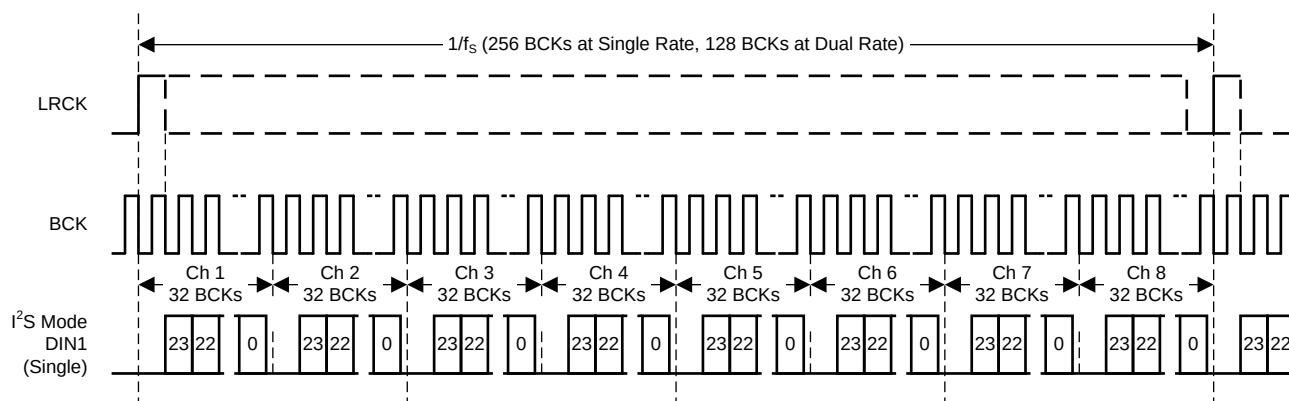
Figure 17. TDM Format
