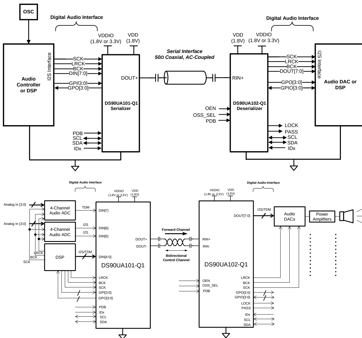
Figure 1. Typical Applications
