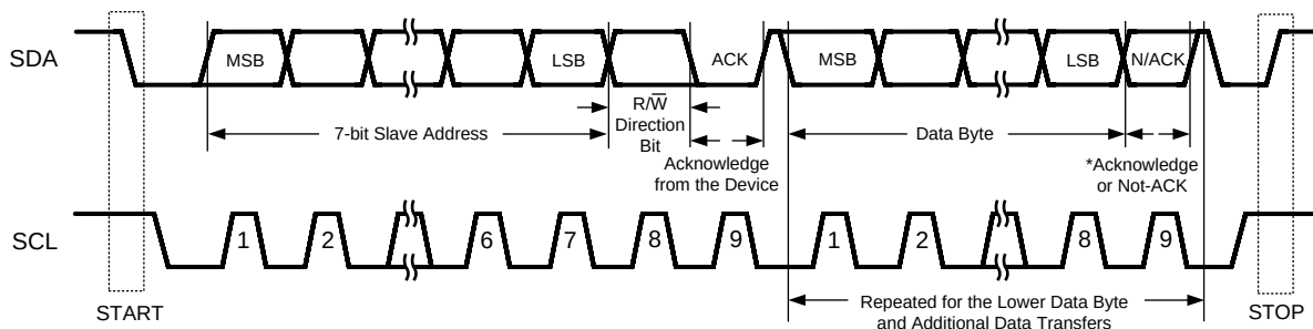
Figure 20. Basic Operation
