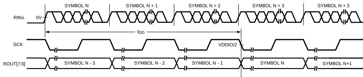
Figure 8. Deserializer Delay
