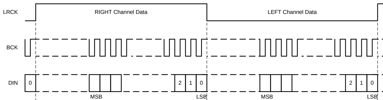
Figure 16. Right-Justified Format
