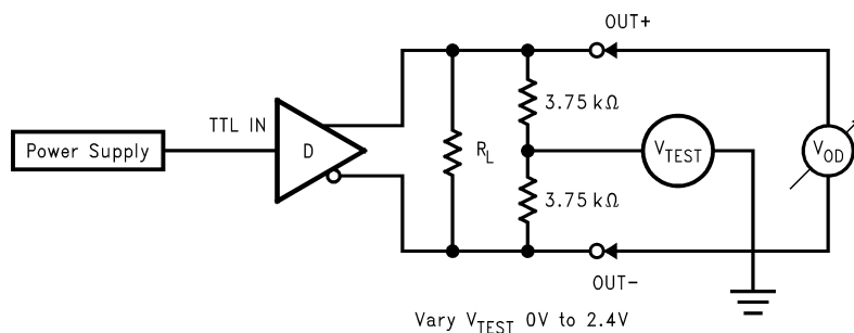
Figure 7-2. Differential Driver Full Load DC Test Circuit
