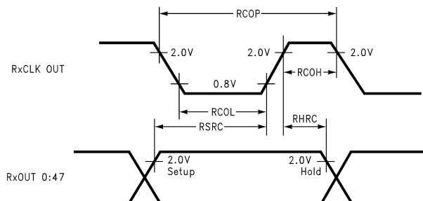
Figure 6. DS90CR482 (Receiver) Setup/Hold and High/Low Times
