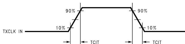
Figure 5. DS90CR217 (Transmitter) Input Clock Transition Time
