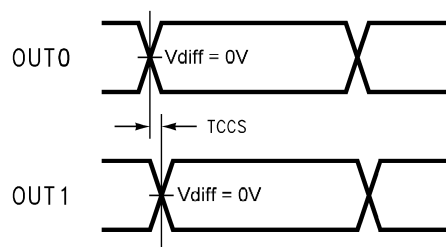
Figure 9. Output Channel-to-Channel Skew in 1:2 splitter mode
