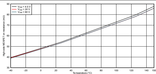
Figure 5-3. High-side FET on resistance
