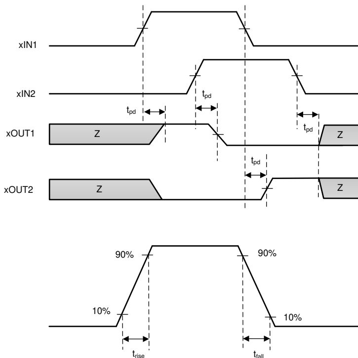
Figure 6-1. Timing Diagram
