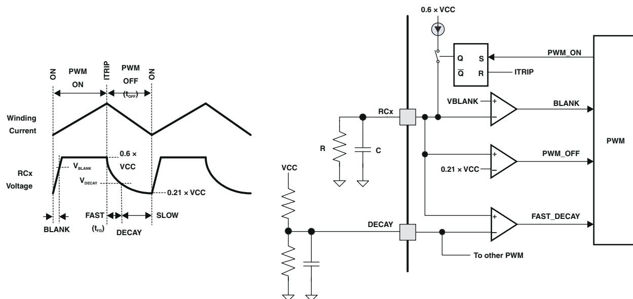
Figure 6-3. PWM
