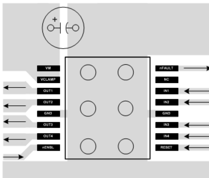
Figure 8-9. Recommended Layout
