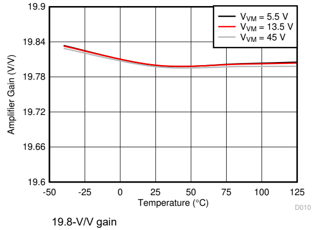
Figure 5-10. Amplifier Gain
