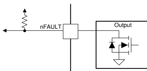
Figure 6-5. nFAULT Block Diagram
