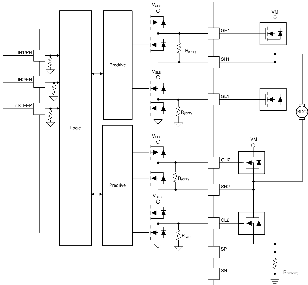
Figure 6-9. Predrive Block Diagram
