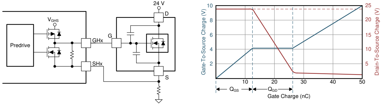
Figure 6-11. FET Gate Charging Profile
