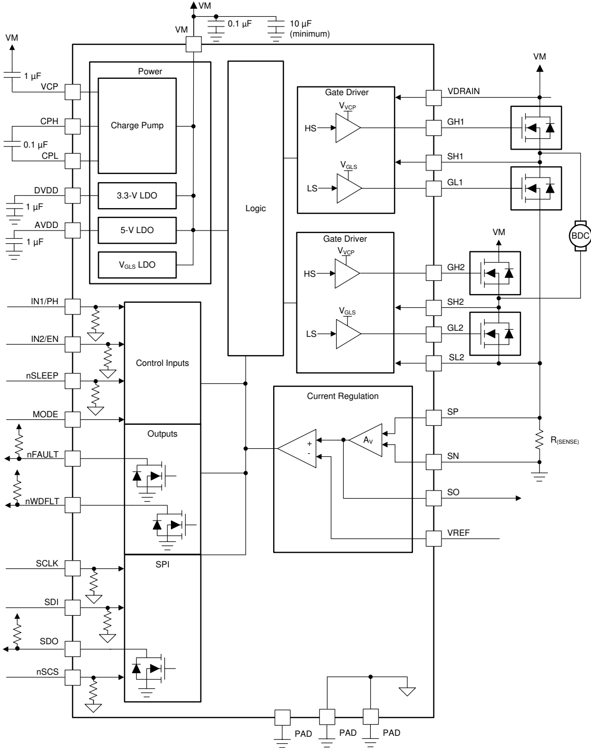
Figure 6-2. DRV8703-Q1 Functional Block Diagram
