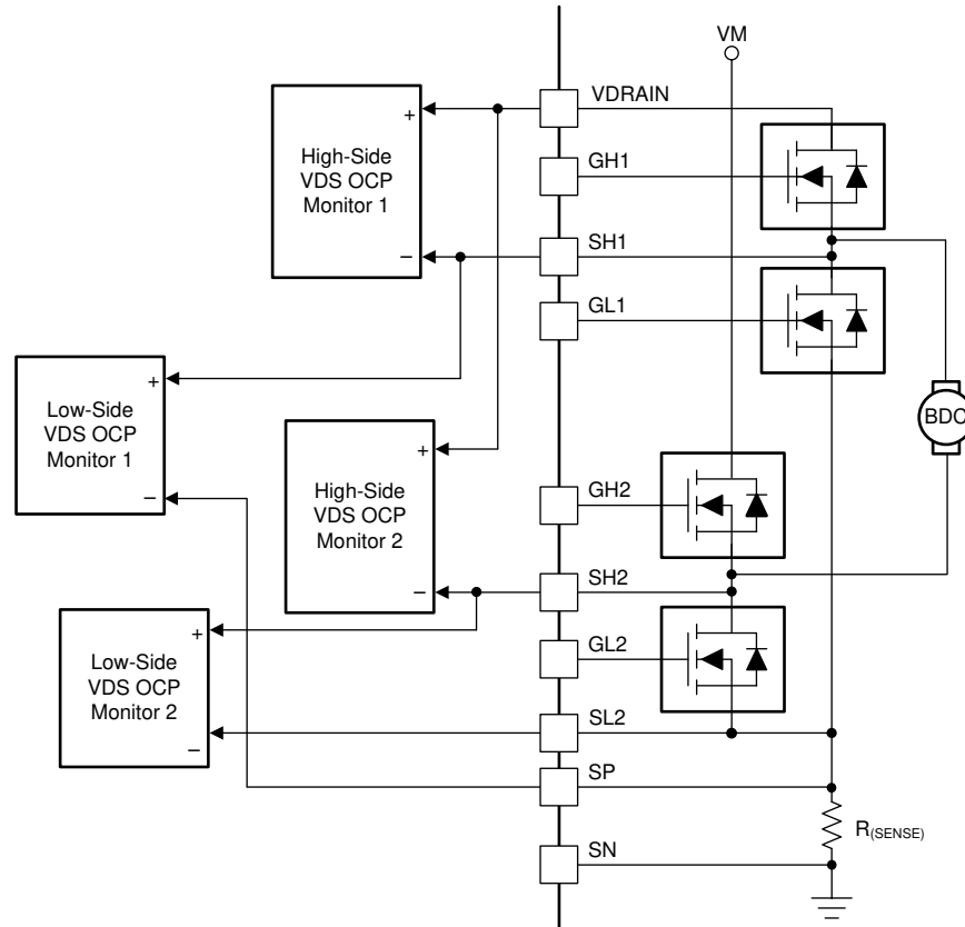
Figure 6-13. V_{DS(OCF)} Block Diagram
