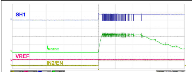
Figure 8-4. Current Profile on Motor Startup With Regulation
