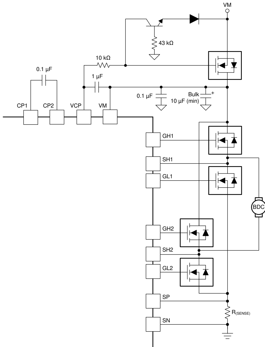
Figure 6-17. Reverse Supply Protection
