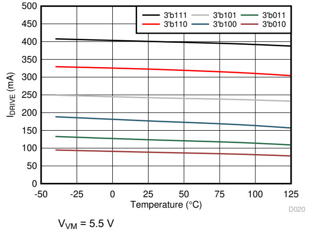
Figure 5-20. High-Side Sink Current
