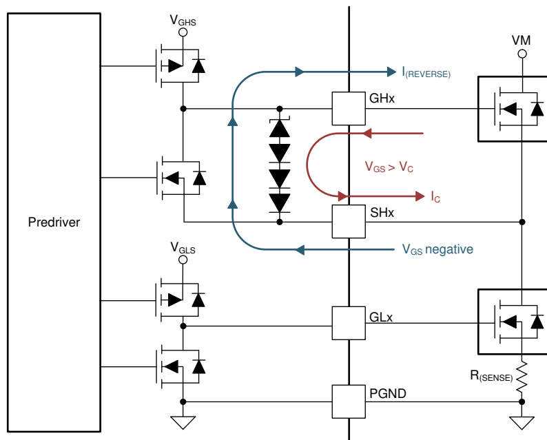
Figure 6-16. Gate Drive Clamp
