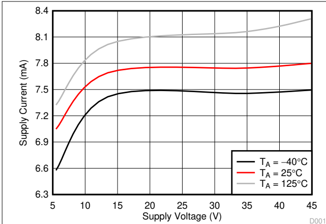
Figure 5-1. Supply Current vs Supply Voltage (VM)
