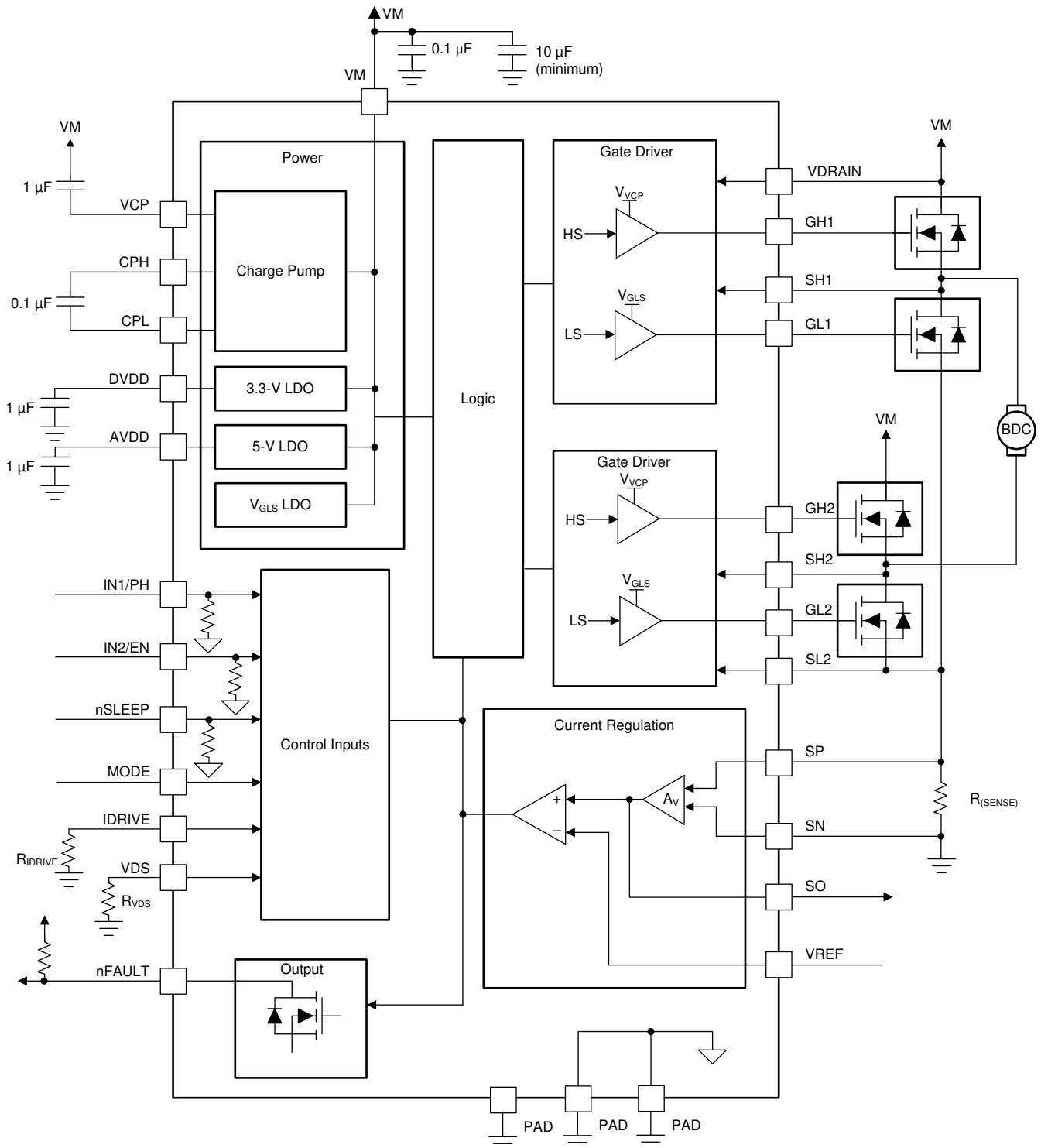
Figure 6-1. DRV8702-Q1 Functional Block Diagram
