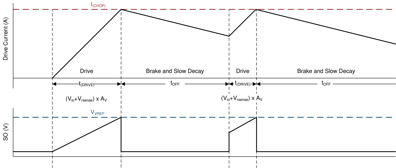
Figure 6-7. Current Sense Amplifier and Current Chopping Operation
