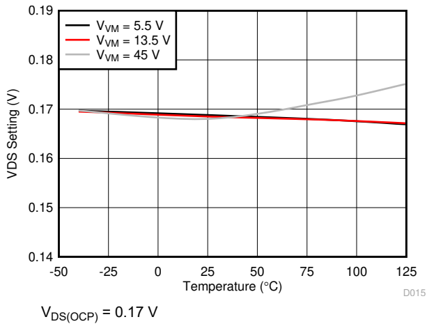
Figure 5-15. OCP Threshold Voltage
