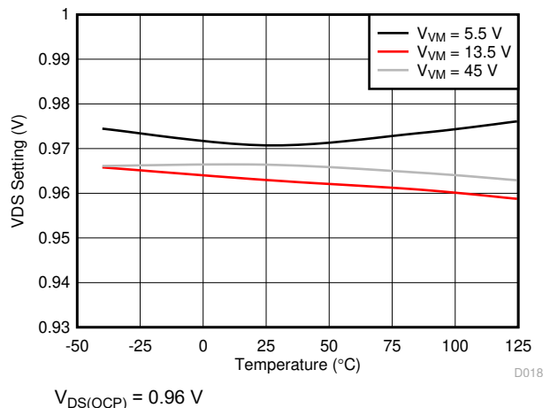
Figure 5-18. OCP Threshold Voltage
