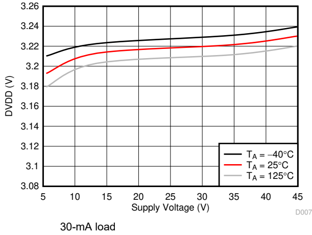
Figure 5-7. DVDD Regulator
