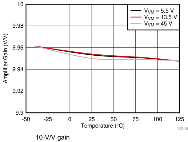
Figure 5-9. Amplifier Gain
