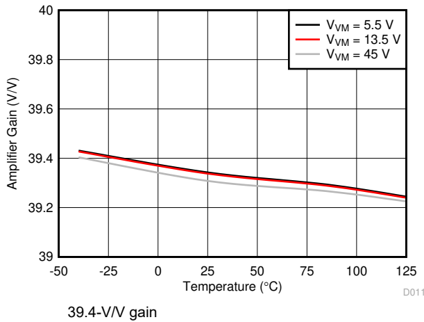
Figure 5-11. Amplifier Gain
