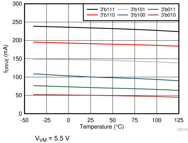
Figure 5-19. High-Side Source Current
