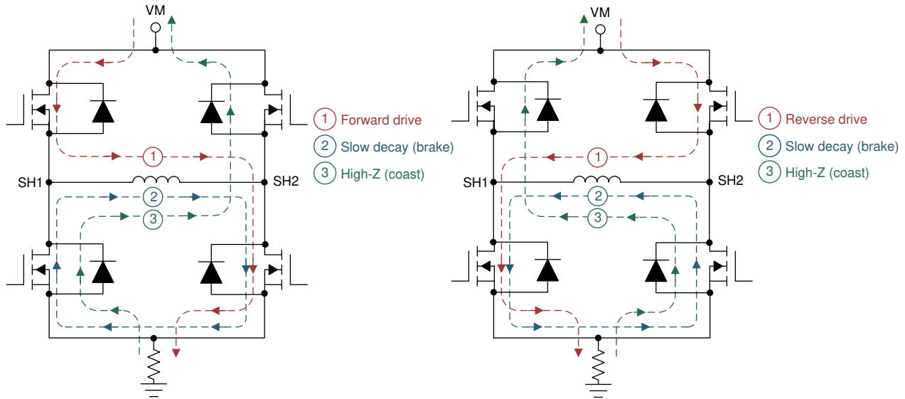
Figure 6-3. Bridge Control
