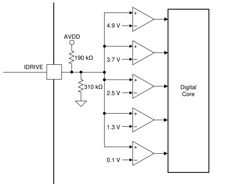
Figure 6-12. IDRIVE Pin Internal Circuitry
