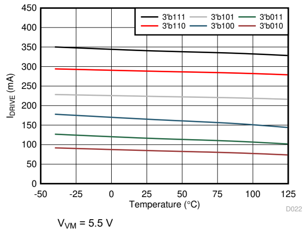
Figure 5-22. Low-Side Sink Current
