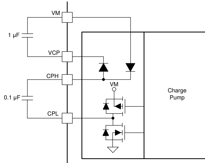
Figure 6-15. Charge Pump Block Diagram
