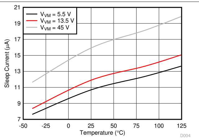
Figure 5-4. Sleep Current vs Temperature
