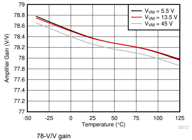
Figure 5-12. Amplifier Gain
