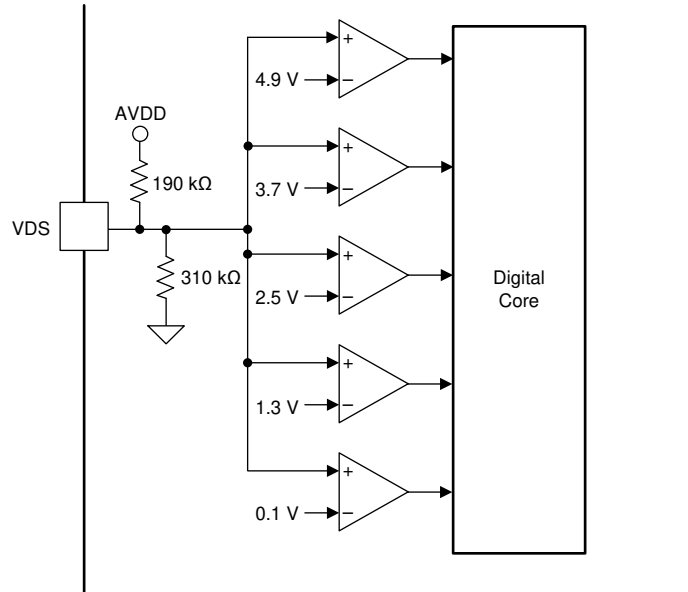
Figure 6-14. VDS Block Diagram
