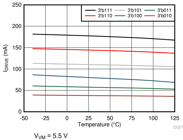
Figure 5-21. Low-Side Source Current
