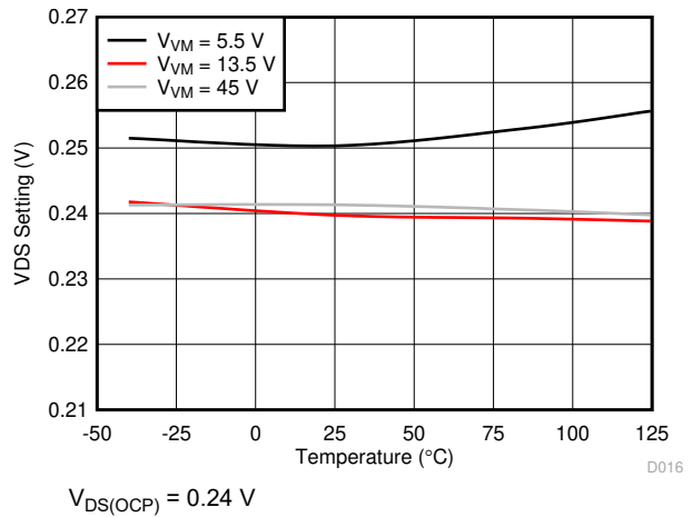
Figure 5-16. OCP Threshold Voltage
