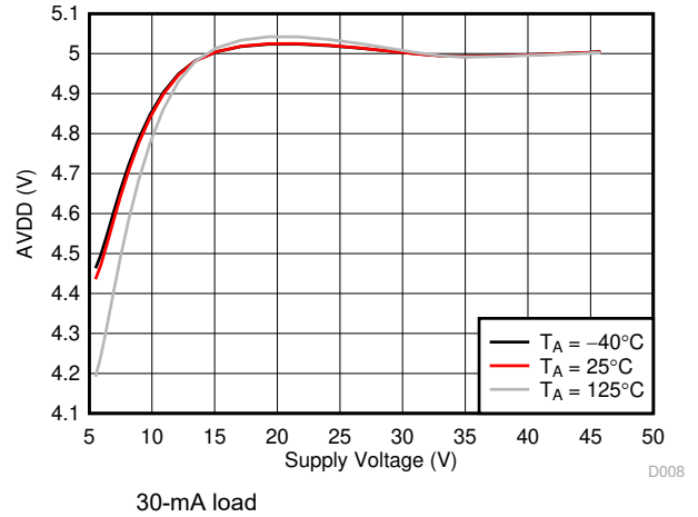
Figure 5-8. AVDD Regulator
