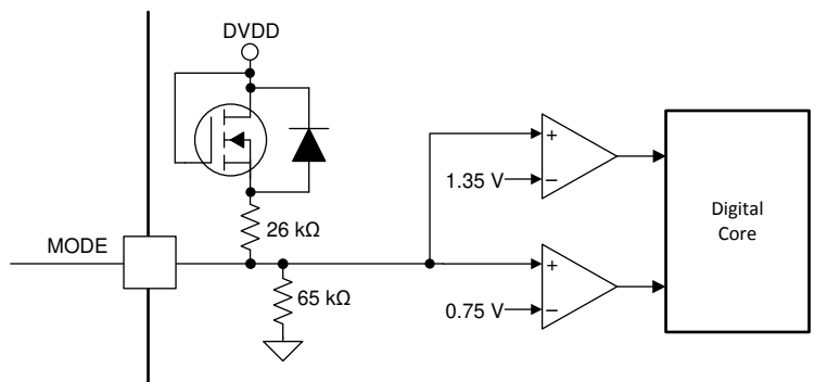
Figure 6-4. MODE Pin Block Diagram
