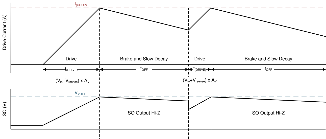
Figure 6-8. Sample and Hold Operation
