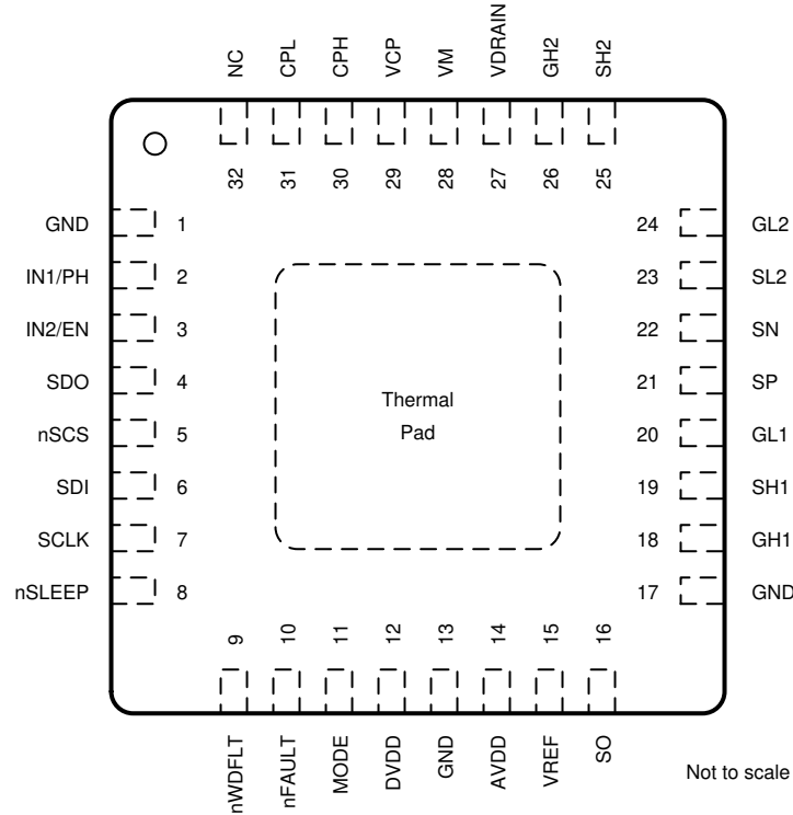
Figure 4-2. DRV8703-Q1 RHB Package With Wettable Flanks 32-Pin VQFN Top View
