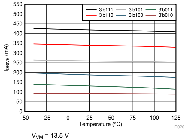
Figure 5-26. Low-Side Sink Current
