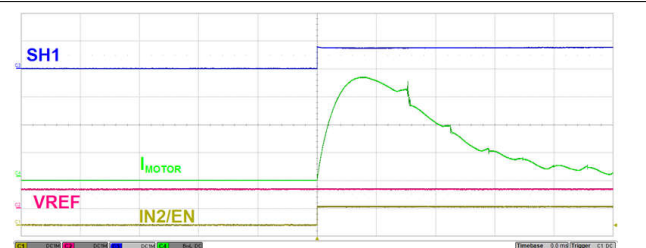
Figure 8-5. Current Profile on Motor Startup Without Regulation
