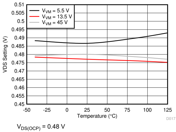
Figure 5-17. OCP Threshold Voltage
