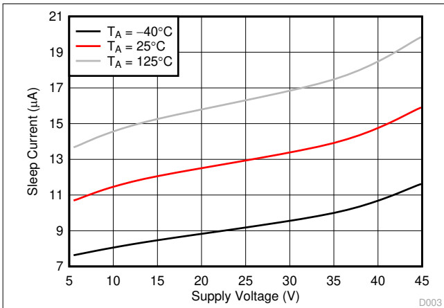
Figure 5-3. Sleep Current vs Supply Voltage (VM)
