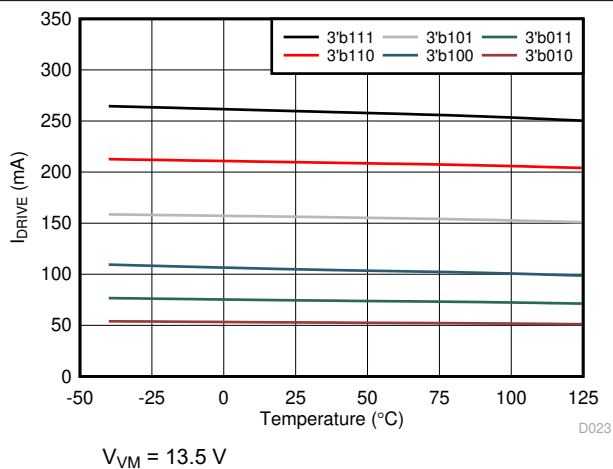
Figure 5-23. High-Side Source Current
