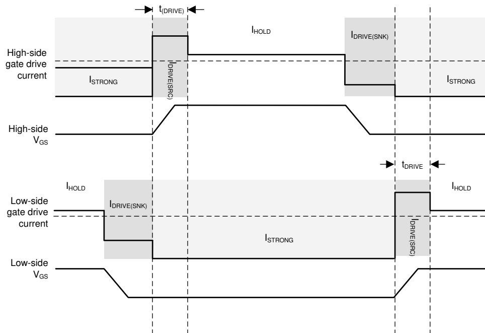
Figure 6-10. Gate Driver Output to Control External FETs
