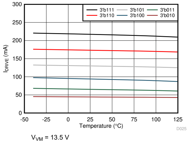
Figure 5-25. Low-Side Source Current
