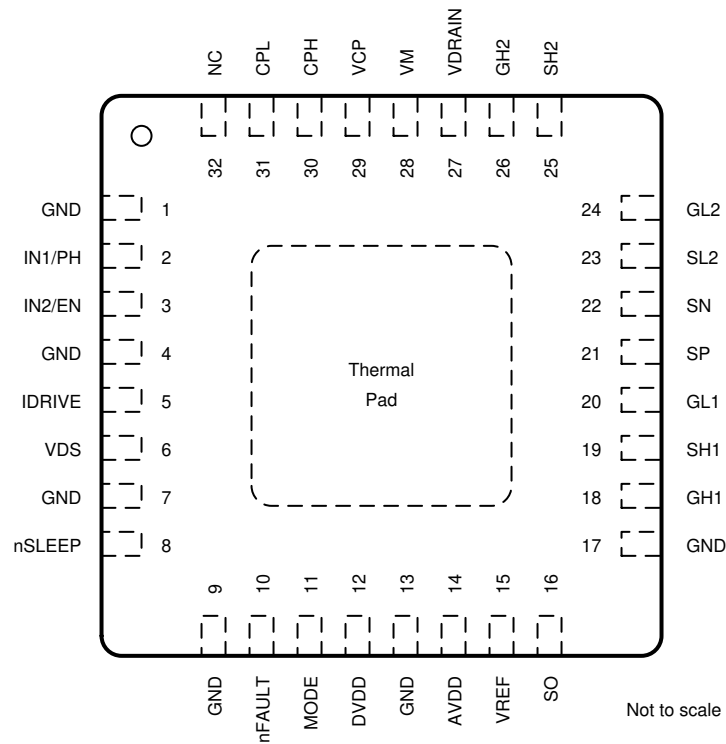
Figure 4-1. DRV8702-Q1 RHB Package With Wettable Flanks 32-Pin VQFN Top View
