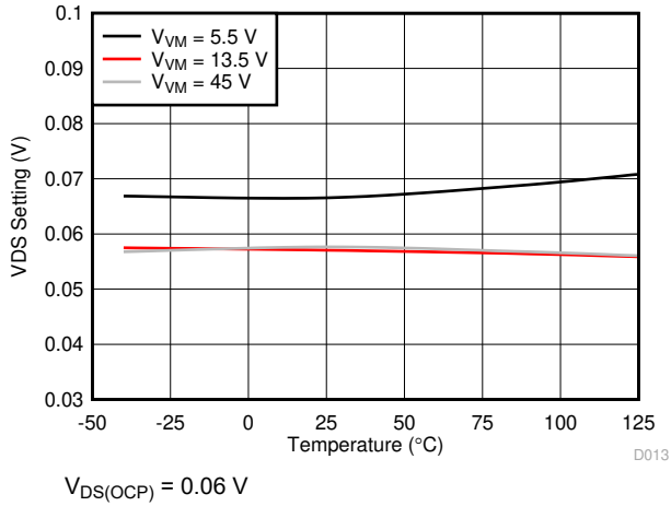
Figure 5-13. OCP Threshold Voltage
