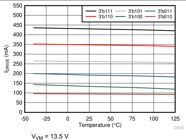
Figure 5-24. High-Side Sink Current
