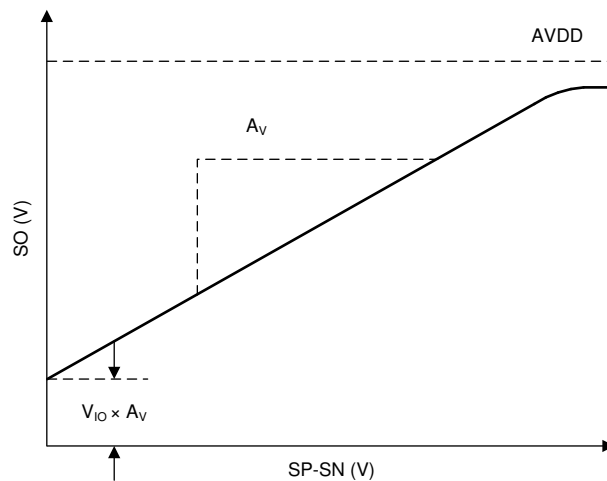
Figure 6-6. Current Sense Amplifier Output
