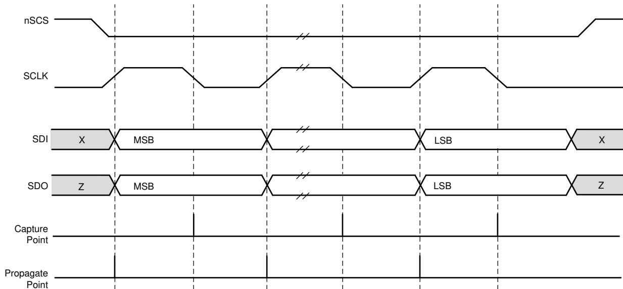
Figure 6-18. SPI Transaction
