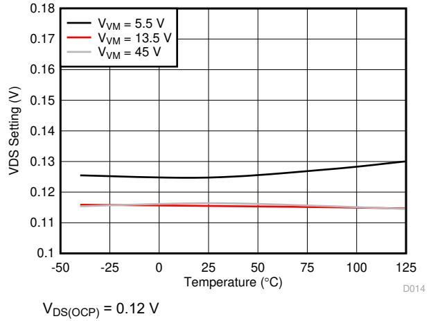
Figure 5-14. OCP Threshold Voltage
