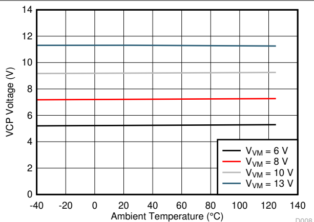
Figure 7-9. VCP Voltage Over Temperature
