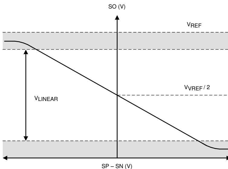
Figure 8-27. Bidirectional Current Sense Output
