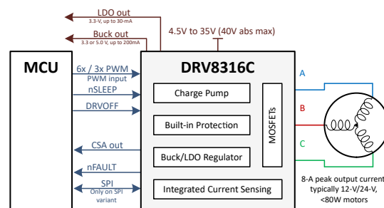
Simplified Schematic
