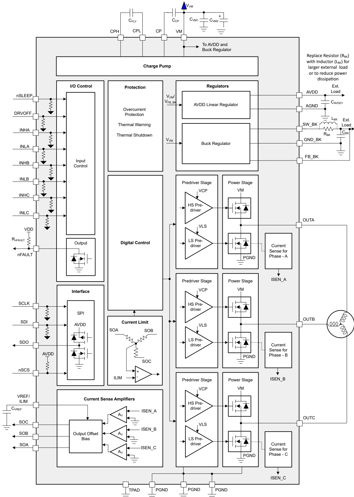
Figure 8-1. DRV8316CR Block Diagram
