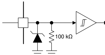
Figure 7-3. Logic-level input
