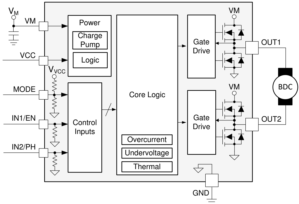
Figure 7-1. DRV8218 Functional Block Diagram
