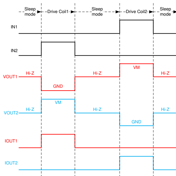
Figure 8-23. Timing diagram for driving a dual-coil relay with PWM interface
