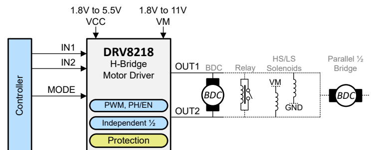
Simplified Schematic
