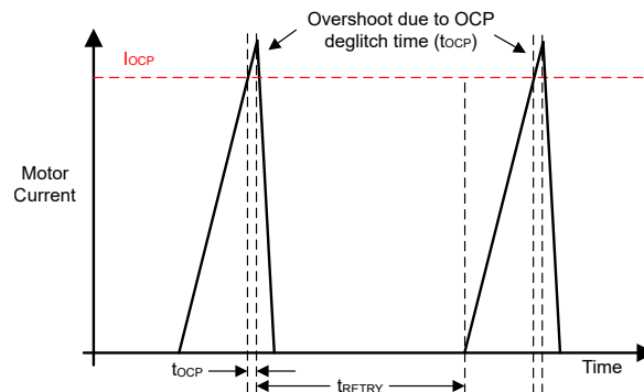
Figure 7-5. OCP Operation
