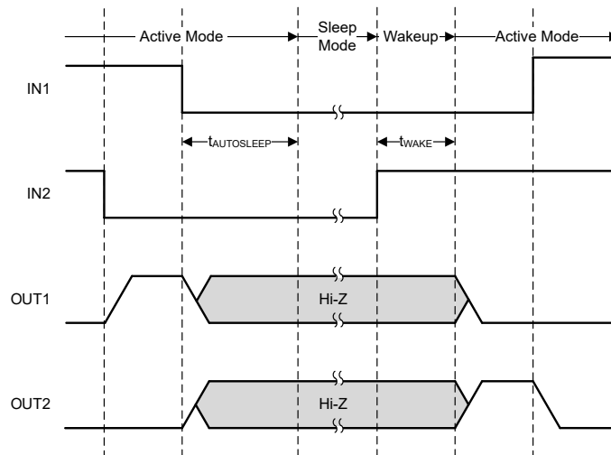
Figure 7-6. Sleep Mode Entry and Wakeup Timing Diagram
