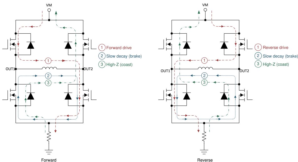
Figure 7-2. H-bridge states
