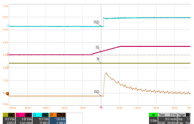
A. Channel 1 = IN1, IN2 (paralleled) Channel 2 = V_{CC} Channel 3 = V_{OUT} (OUT1/2paralleled) Channel 8 = Motor Current
