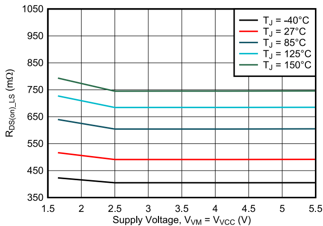
Figure 7-13. Low-Side R_{DS(on)} vs. Supply Voltage
