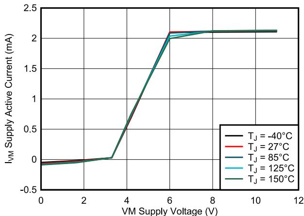
Figure 7-5. Active Current ( I_{VM} ) vs. Supply Voltage ( V_{VM} )
