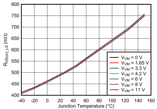
Figure 7-14. Low-Side R_{DS(on)} vs. Junction Temperature ( T_J )
