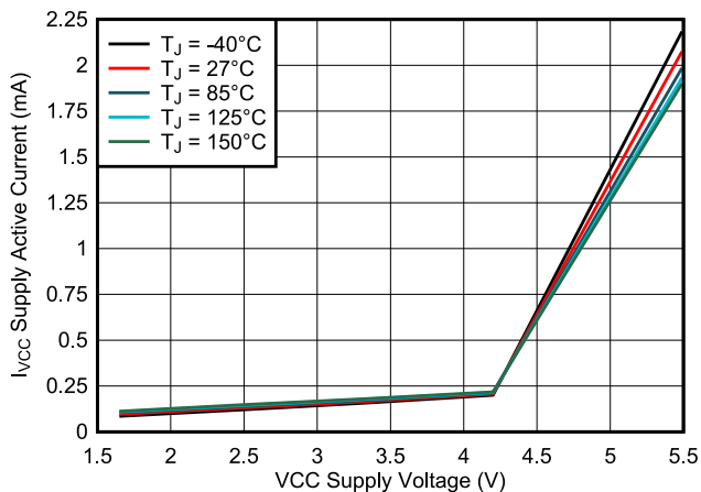
Figure 7-7. Active Current ( I_{VCC} ) vs. Supply Voltage ( V_{VCC} )
