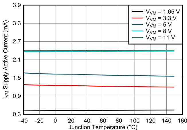
Figure 7-20. Active Current ( I_{VM} ) vs. Junction Temperature ( T_J )
