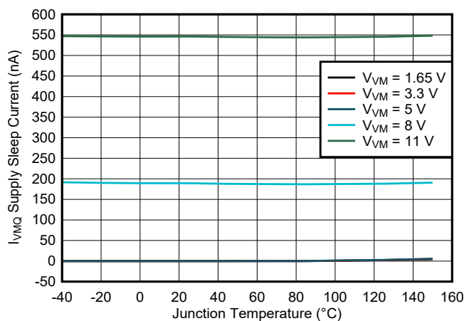
Figure 7-18. Sleep Current ( I_{VMQ} ) vs. Junction Temperature ( T_J )
