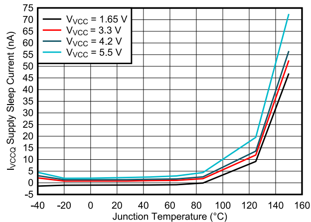
Figure 7-4. Sleep Current ( I_{VCCQ} ) vs. Junction Temperature ( T_J )
