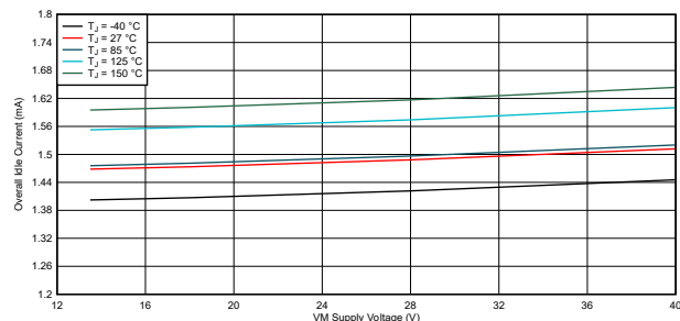
Figure 6-2. Idle mode supply current, VDD = 5.5V
