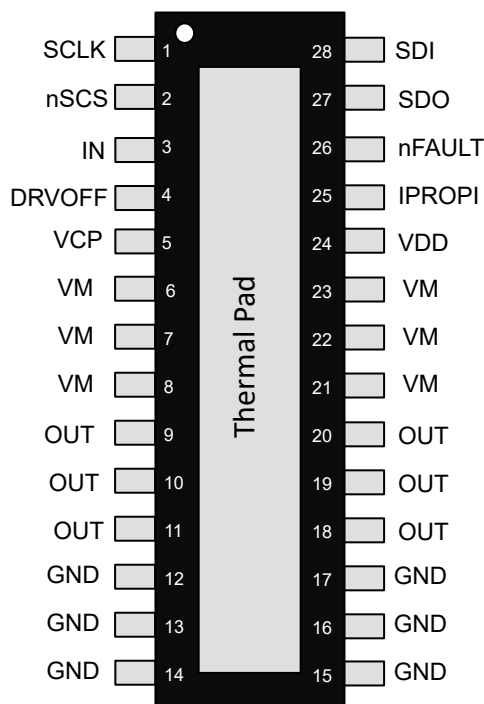
Figure 5-2. DRV8145P-Q1 SPI(P) variant in HTSSOP (28) package
