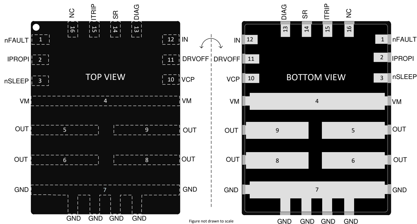
Figure 5-1. DRV8145H-Q1 HW variant in VQFN-HR(16) package
