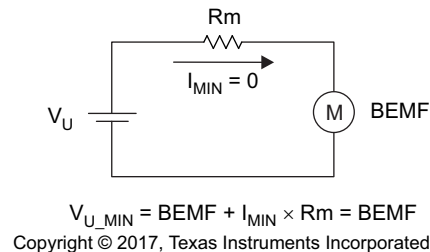
Figure 39. Mechanical AVS
