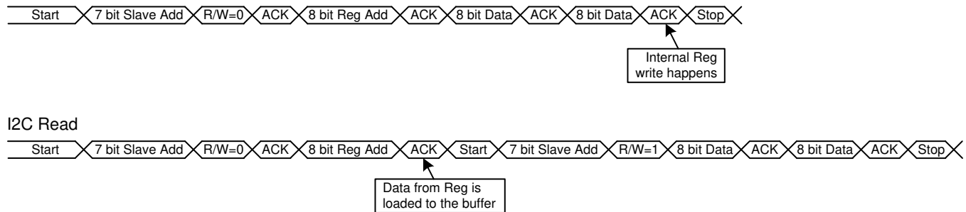
Figure 45. I 2 C Protocol
