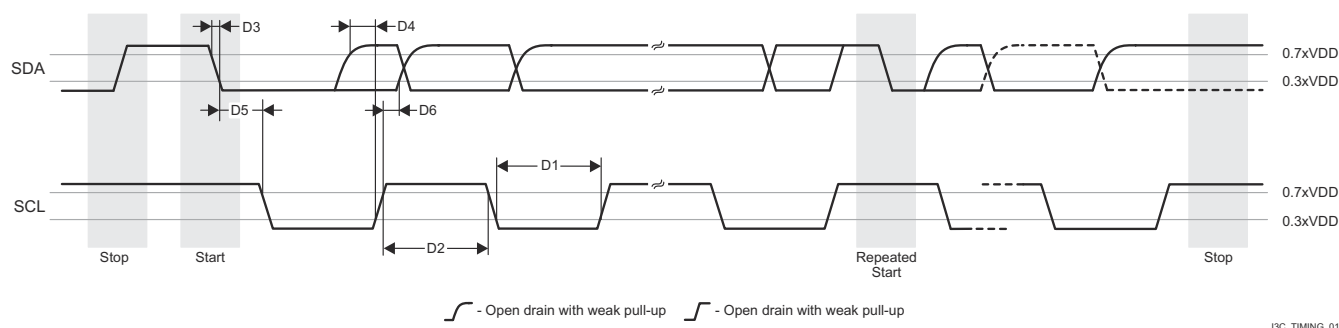
Figure 6-77. I3C Open Drain Timing
