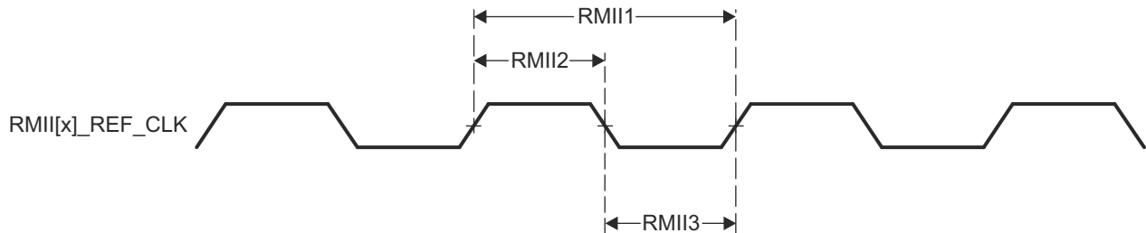
Figure 6-47. RMII[x]_REFCLK Timing – RMII Mode
