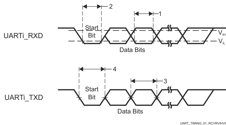
Figure 6-114. UART Timing
