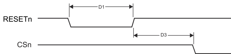
Figure 6-75. HyperBus Timing Diagrams – Receiver Mode
