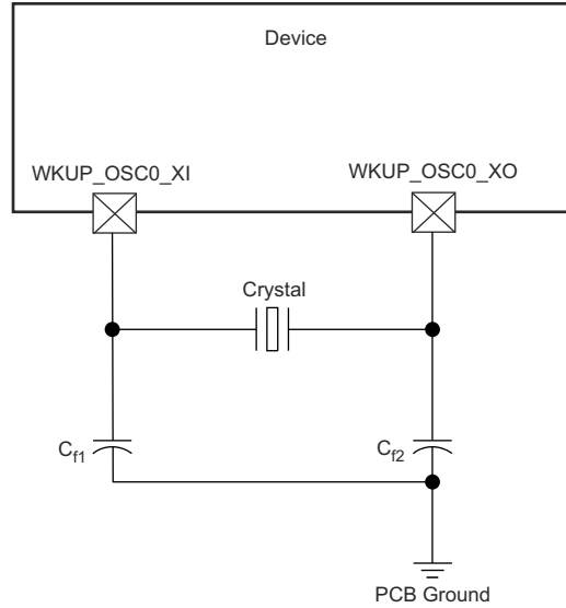
Figure 6-26. WKUP_OSC0 Crystal Implementation
