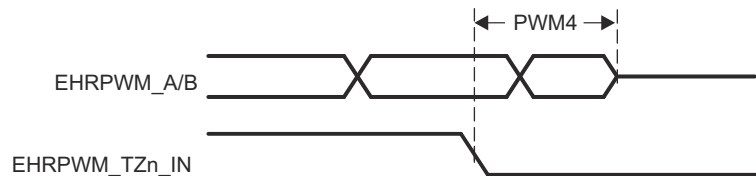
Figure 6-56. EPWM_A/B and ePWM_TZn_IN Hi-Z Input Timings
