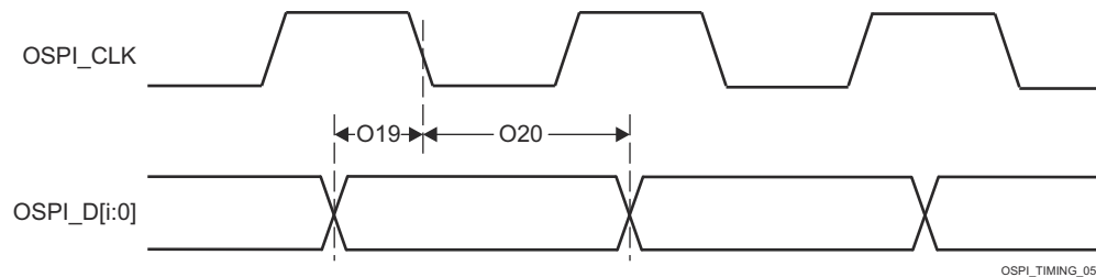
Figure 6-111. OSPI Timing Requirements – SDR, No Loopback Clock and Internal Pad Loopback Clock
