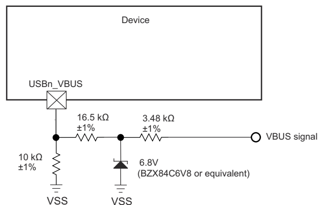
Figure 8-5. USB VBUS Detect Voltage Divider / Clamp Circuit
