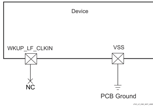
Figure 6-39. WKUP_LF_CLKIN Not Used
