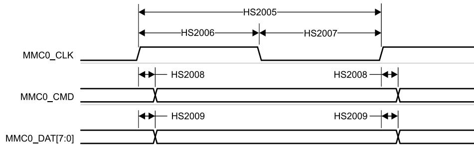
Figure 6-92. MMCSD0 – HS200 Mode – Transmit Mode
