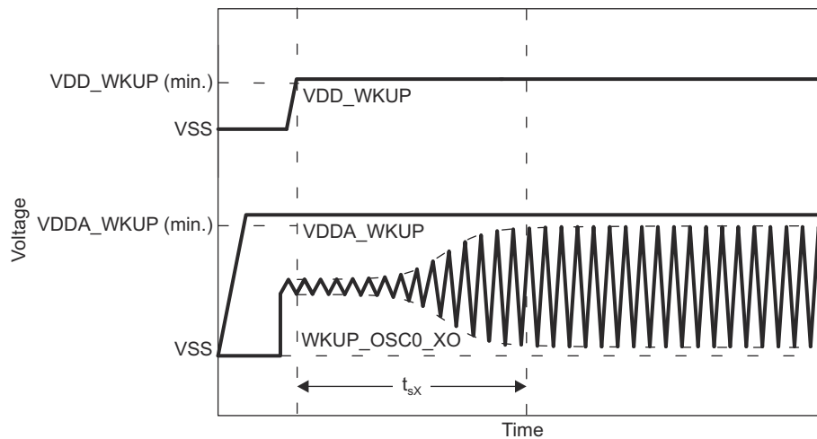
Figure 6-27. WKUP_OSC0 Start-up Time
