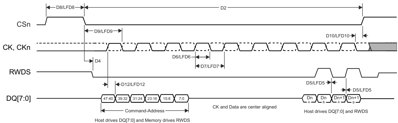
Figure 6-74. HyperBus Timing Diagrams – Transmitter Mode
