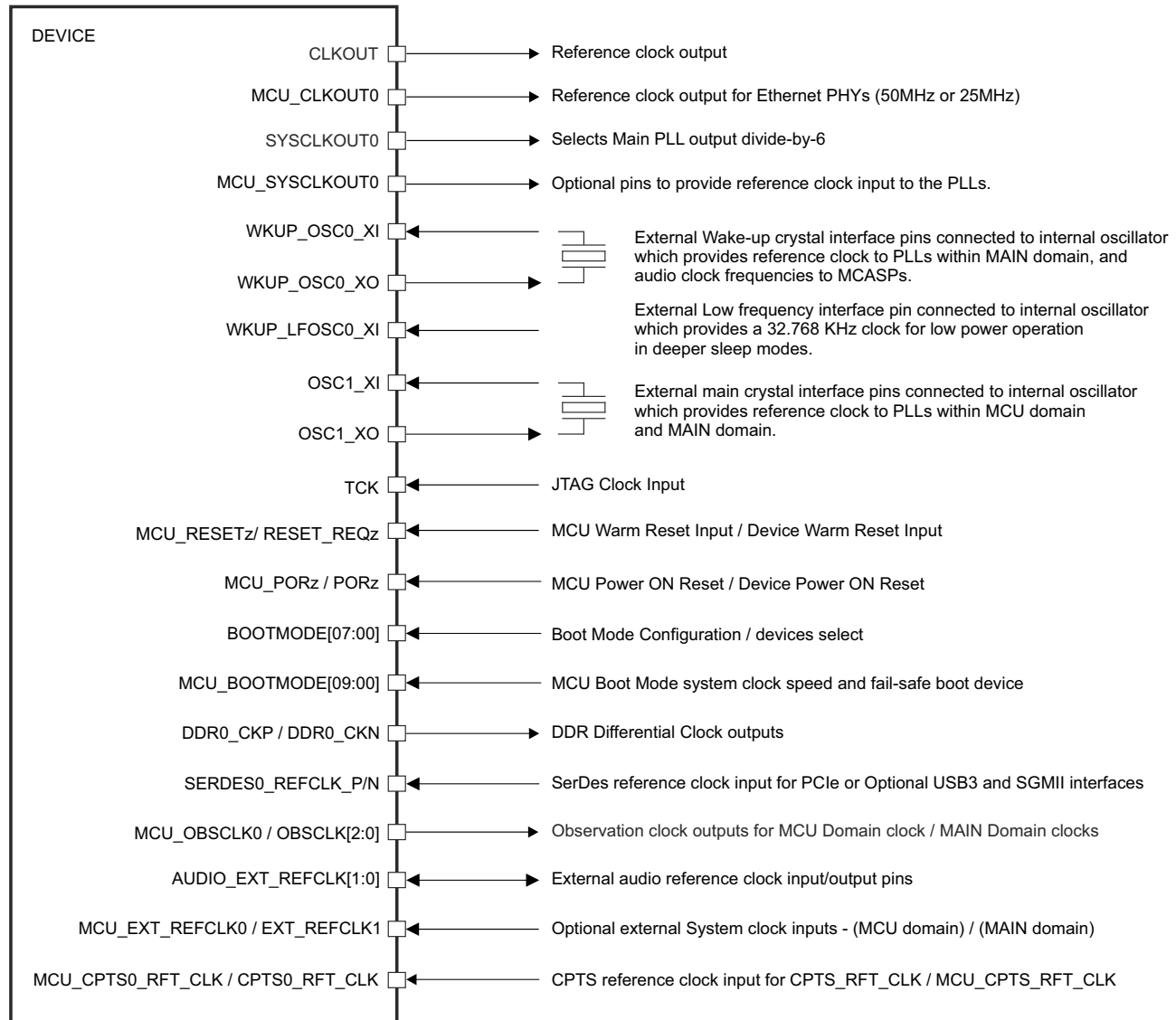
Figure 6-25. Input Clocks Interface
