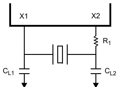
Figure 6-3. Crystal Oscillator Circuit
