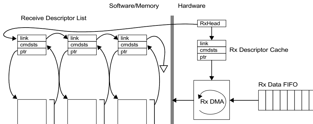
Figure 5-22. Receive Architecture
