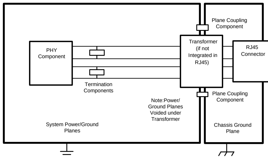
Figure 8-5. Layout Example
