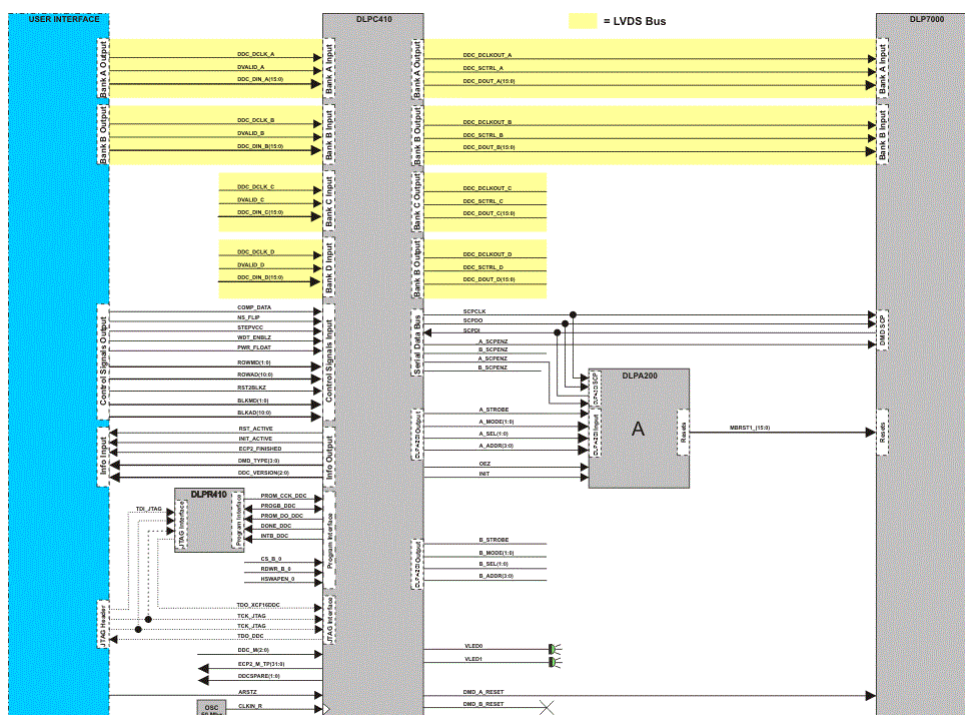
Figure 8-1. DLPC410 and DLP7000 Chipset Block Diagram
