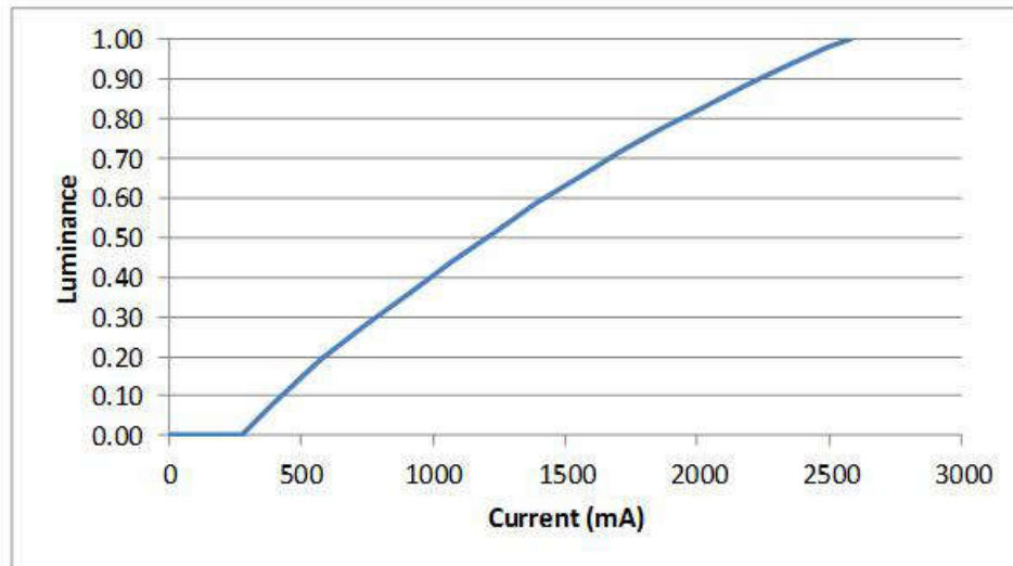
Figure 7-2. Luminance vs Current
