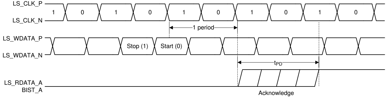
Figure 5-2. Switching Characteristics
