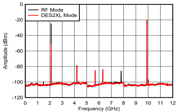
Figure 6-22. f_{\text{OUT}} = 8097\text{MHz} , -12dBFS
