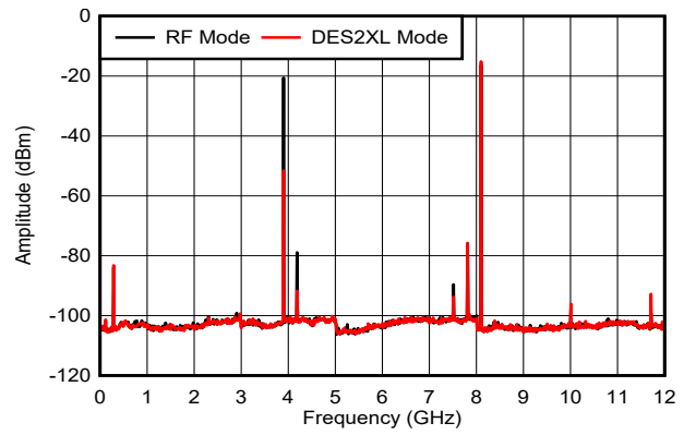
Figure 6-21. f_{\text{OUT}} = 8097\text{MHz} , -6dBFS
