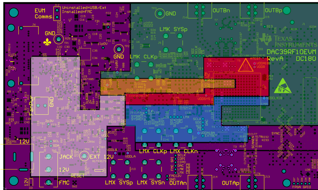
Layer12 / PWR3 DAC VDDA18A = RED DAC VDDA18B = ORANGE DAC VDDB = YELLOW DAC VEXa = GREEN DAC VEXb = BLUE VDDIO = WHITE Figure 8-32. Power Plane Layout for Layer 12
