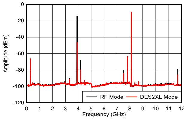
Figure 6-20. f_{\text{OUT}} = 8097\text{MHz} , 0dBFS
