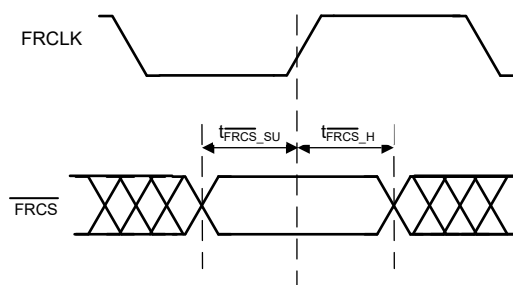
Figure 6-7. \overline{FRCS} Timing Diagram
