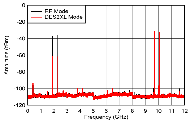
Figure 6-41. Dual Tone, f_{\text{OUT}} = 9897\text{MHz} , 0dBFS
