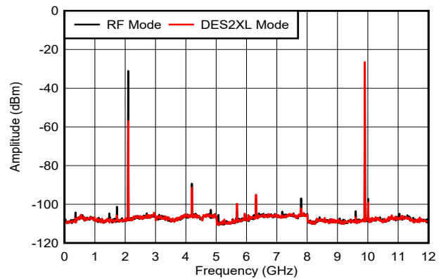
Figure 6-23. f_{\text{OUT}} = 9897\text{MHz} , 0dBFS
