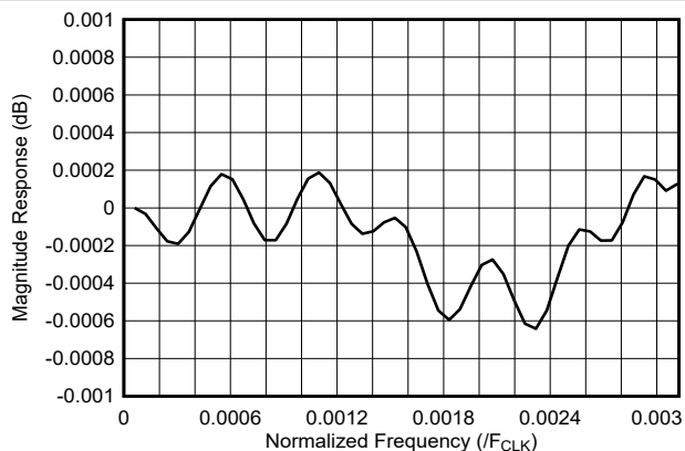
Figure 7-39. 128x Interpolation Filter Passband Response
