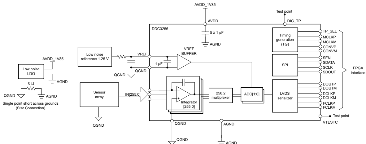
Simplified Schematic
