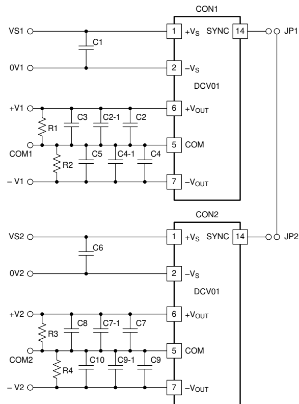
Figure 11-1. PCB Schematic, P and U Package
