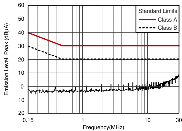
Figure 7-1. Conducted Emissions
