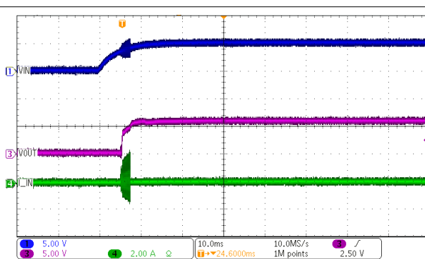
Figure 8-4. DCV010505P Start-Up at 10% Load
