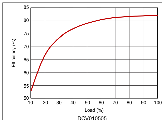
Figure 9-3. Efficiency versus Load
