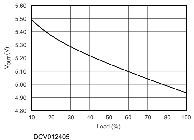
Figure 7-18. Load Regulation
