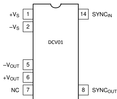
Figure 6-1. NVA, DUA Package 7-Pin PDIP, SOP (Single-Output) (Top View)
