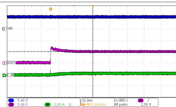
Figure 8-6. DCV010505P Enable Start-Up at 100% Load
