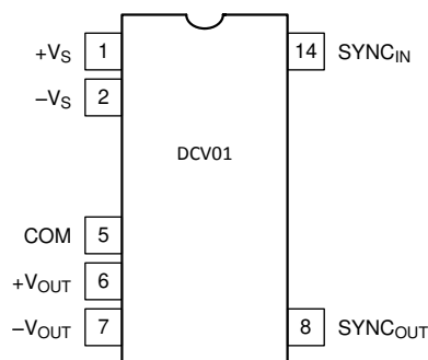
Figure 6-2. NVA, DUA Package 7-Pin PDIP, SOP (Dual-Output) (Top View)
