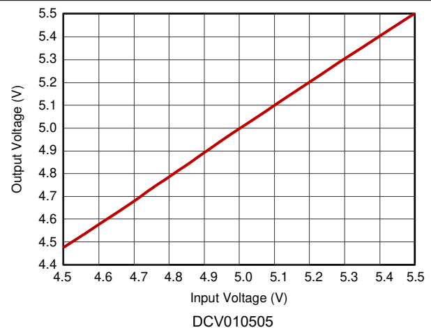
Figure 7-4. Line Regulation
