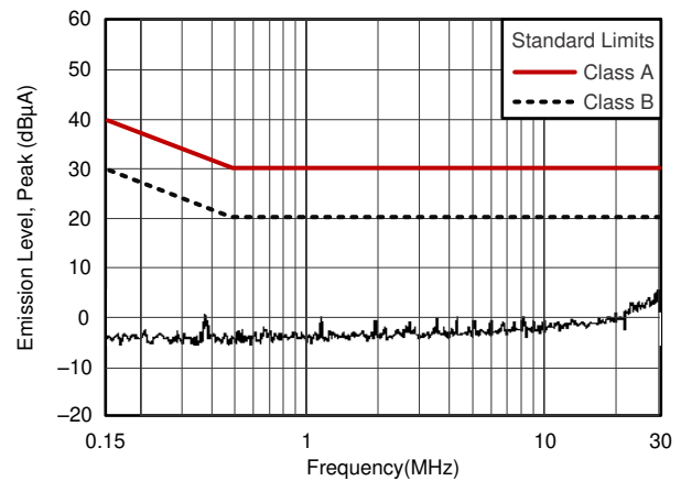
Figure 7-2. Conducted Emissions
