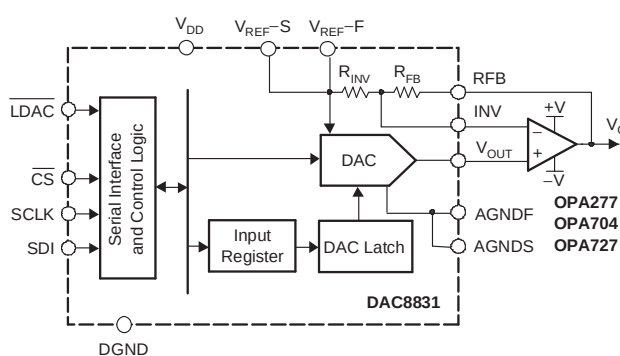
DAC8831 Functional Block Diagram
