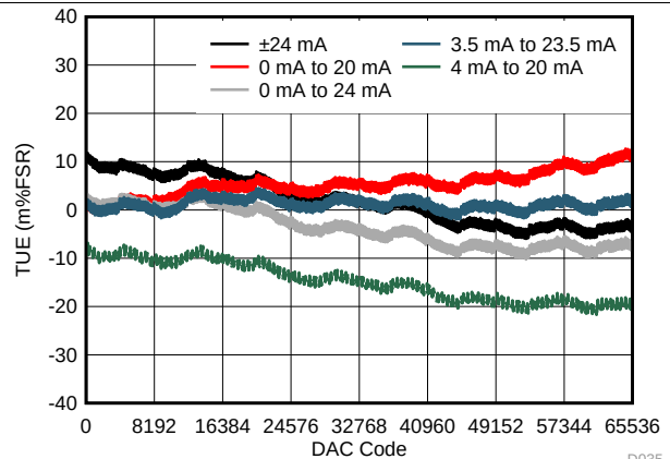
Figure 39. IOUT TUE vs Code (DC/DC Enabled)
