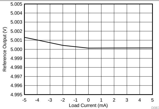
Figure 72. Internal Reference Voltage vs Load
