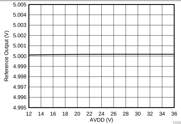
Figure 73. Internal Reference Voltage vs AVDD
