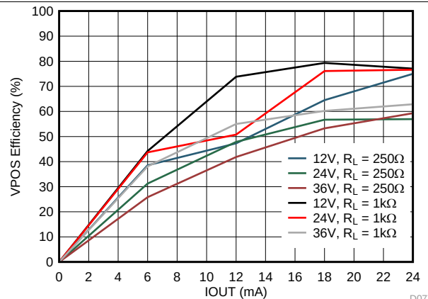
Figure 79. IOU T VPOS Efficiency
