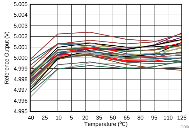
Figure 71. Internal Reference Voltage vs Temperature
