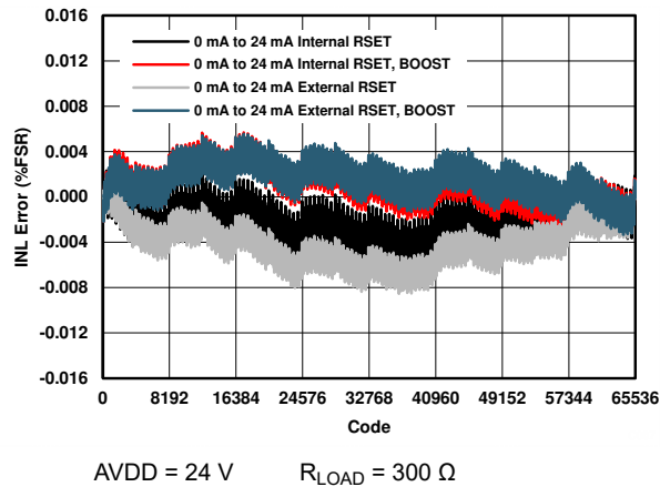
Figure 7-21. IOUT INL vs Code (0 mA to 24 mA)
