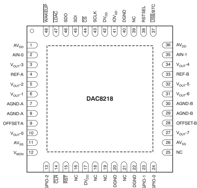
RGZ PACKAGE QFN-48 (TOP VIEW)
