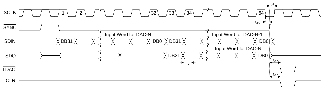
Figure 2. Daisy-Chain Timing
