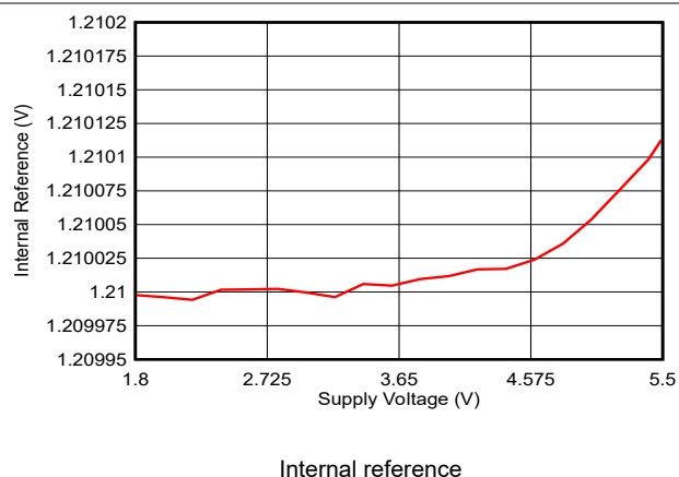
Figure 5-55. Internal Reference vs Supply Voltage
