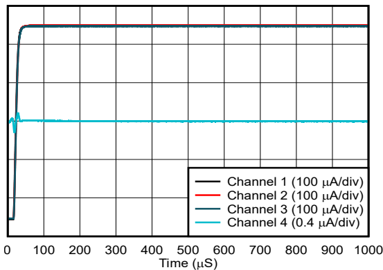
Figure 5-45. Current Output Power-On Glitch
