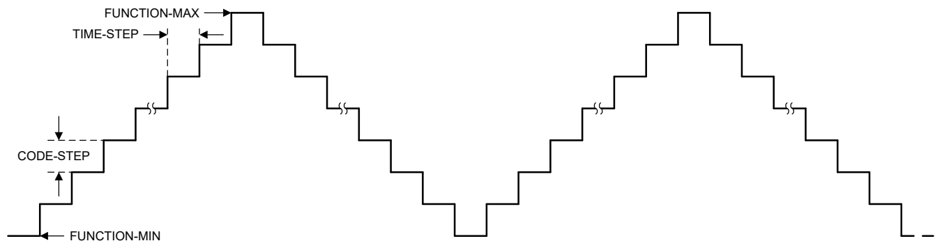
Figure 6-12. Triangle Waveform
