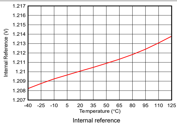
Figure 5-54. Internal Reference vs Temperature
