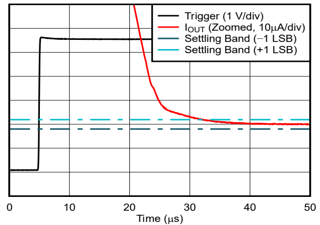
Figure 5-44. Current Output Settling Time: Falling Edge (1/4 to 3/4 scale)
