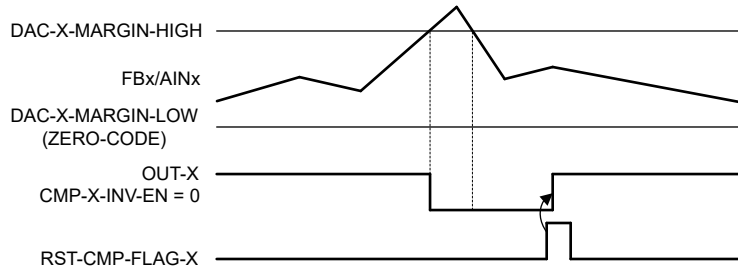
Figure 6-6. Latching Comparator With Active Low Output
