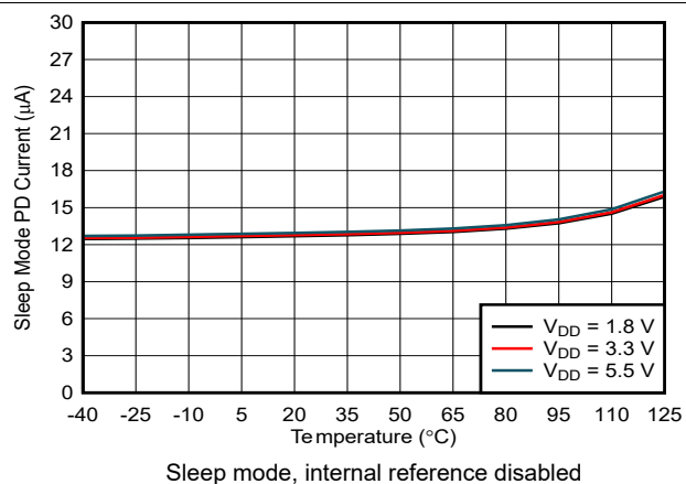
Figure 5-56. Power-Down Current vs Temperature
