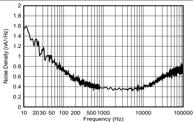
Figure 5-49. Current Output Noise Density
