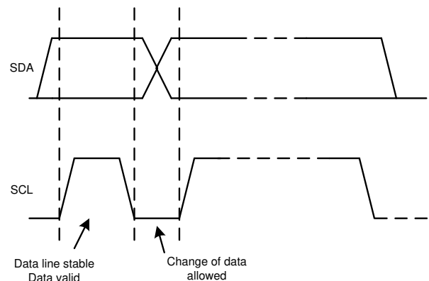
Figure 6-22. Bit Transfer on the I 2 C Bus
