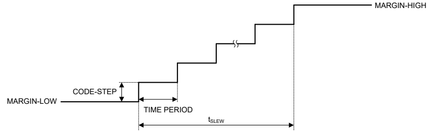
Figure 6-10. Programmable Slew-Rate Control
