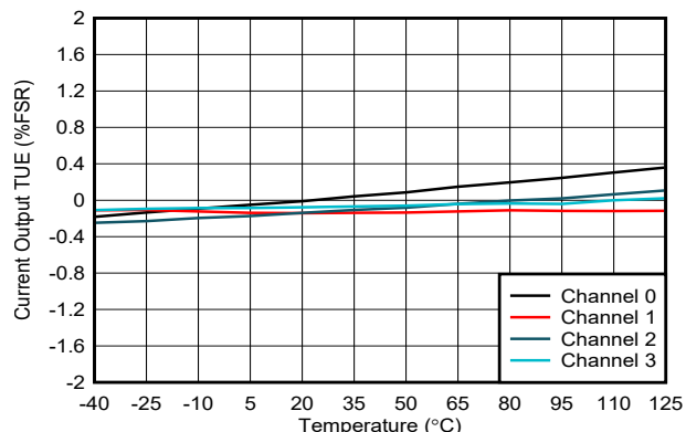
Figure 6-38. Current Output TUE vs Temperature
