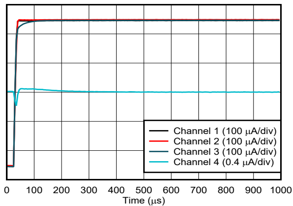
Channel 4 is victim, all other channels are aggressors Figure 6-53. Current Output Channel-to-Channel Crosstalk
