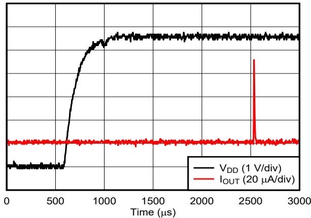
DAC at mid scale (0 \mu\text{A} ) stored in EEPROM Figure 6-51. Current Output Power-On Glitch
