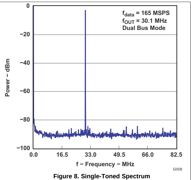
Figure 8. Single-Tone Spectrum
