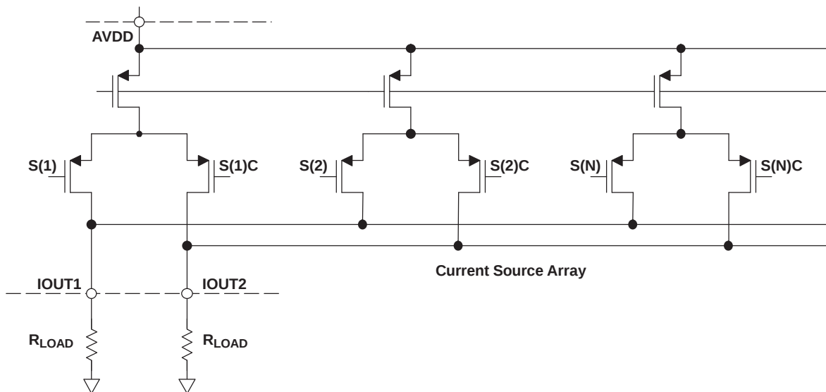
The signal voltage swing that may develop at the two outputs, IOUT1 and IOUT2, is limited by a negative and positive compliance. The negative limit of -1\text{ V} is given by the breakdown voltage of the CMOS process and exceeding it compromises the reliability of the DAC5672 (or even causes permanent damage). With the full-scale output set to 20\text{ mA} , the positive compliance equals 1.2\text{ V} . Note that the compliance range decreases to about 1\text{ V} for a selected output current of I_{\text{OUTFS}} = 2\text{ mA} . Care must be taken that the configuration of DAC5672 does not exceed the compliance range to avoid degradation of the distortion performance and integral linearity.
