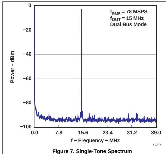
Figure 7. Single-Tone Spectrum
