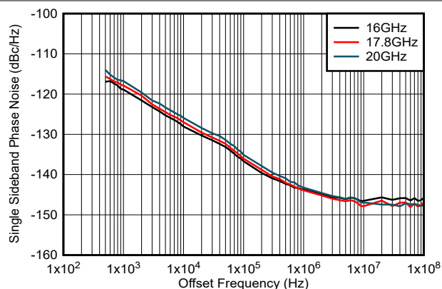
Figure 6-22. Phase Noise in DES2XH Mode, DEM/Dither On
