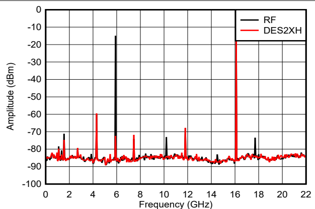
Figure 6-16. Output Spectra at 16097MHz, DEM/Dither Off
