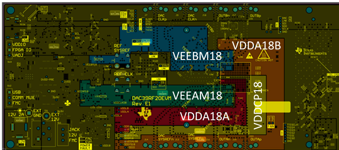
Figure 9-17. Power Plane Layout for Layer 12
