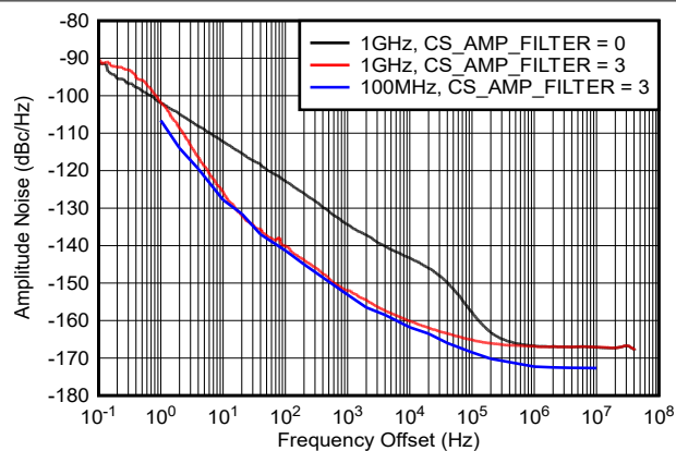
Figure 6-29. AC Amplitude Noise at 1GHz
