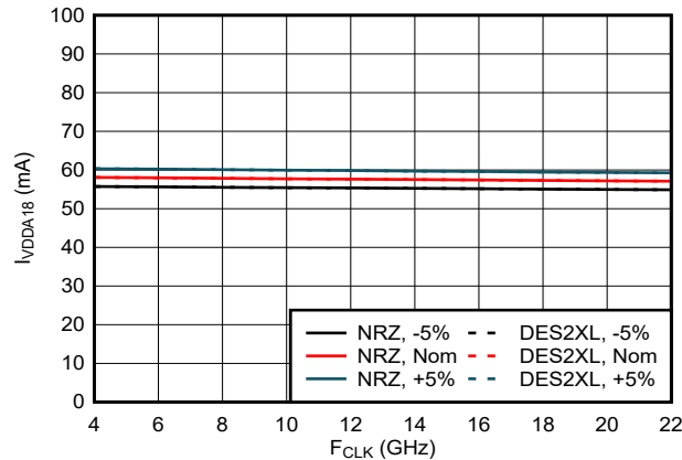
Figure 6-45. I_{VDDA18} vs Input Clock
