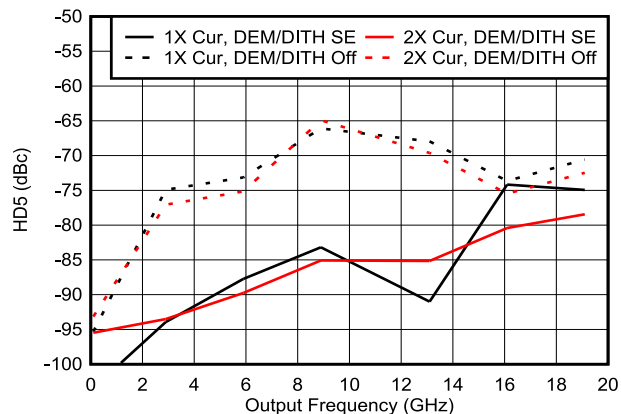
Figure 6-40. HD5 vs Output Frequency in DES2XL and DES2XH Modes
