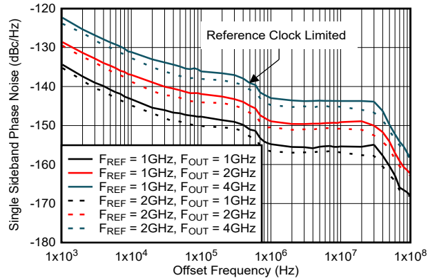
Figure 6-27. Phase Noise with PLL/VCO, NRZ and DEM/Dither off
