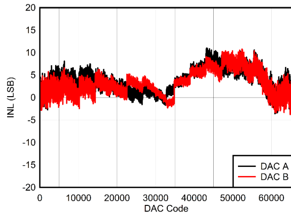
Figure 6-7. Integral Non-Linearity (INL) vs DAC Code
