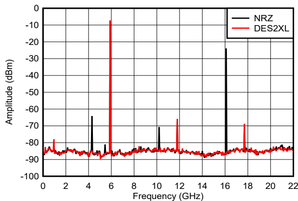
Figure 6-13. Output Spectra at 5897MHz, DEM/Dither On
