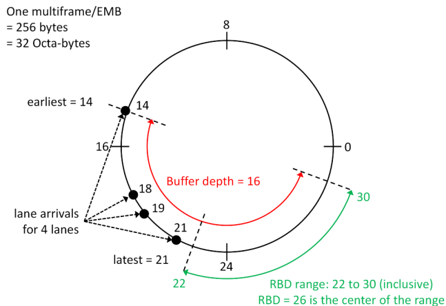
Figure 7-55. RBD Example (lane arrivals do not straddle zero)
