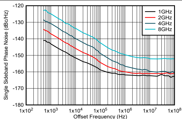
Figure 6-18. Phase Noise in DES2XL Mode, DEM/Dither On
