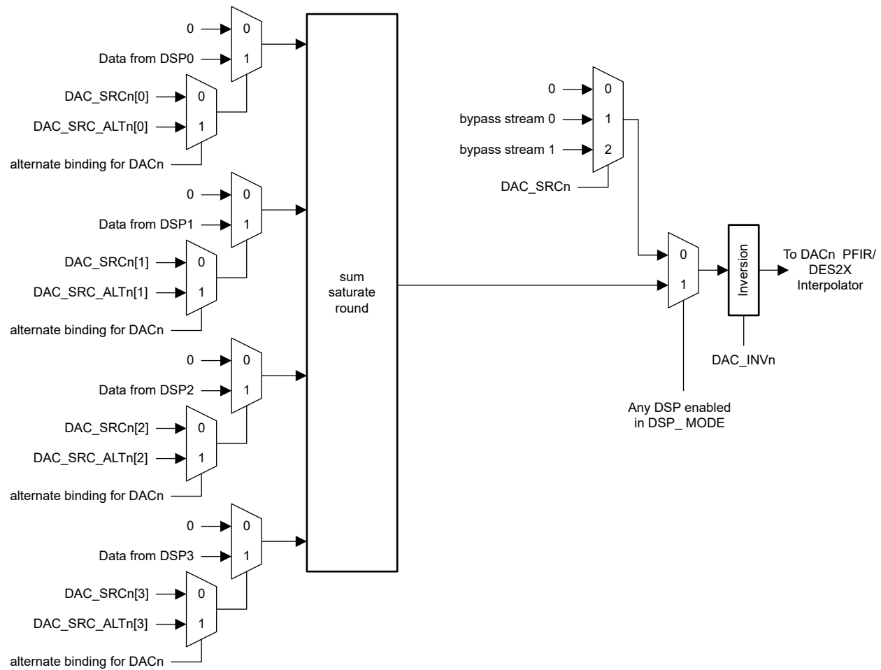
Figure 7-45. Channel Bonder Block Diagram for DAC Channel n
