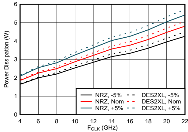
Figure 6-43. Power Dissipation vs Input Clock
