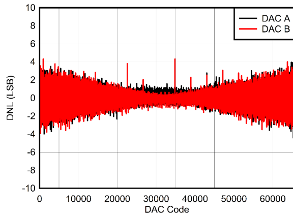
Figure 6-6. Differential Non-Linearity (DNL) vs DAC Code
