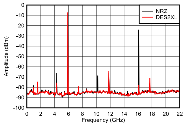
Figure 6-14. Output Spectra at 5897MHz, DEM/Dither Off
