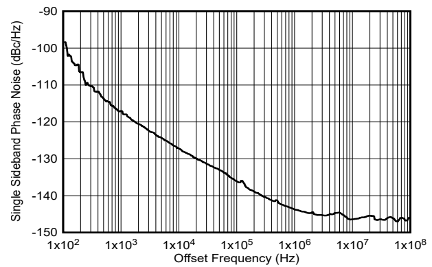
Figure 9-8. DAC Additive Phase Noise at 16.2GHz
