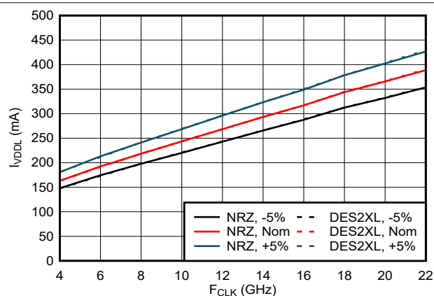
Figure 6-49. I_{VDD} vs Input Clock
