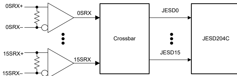
Figure 7-52. Crossbar Block Diagram
