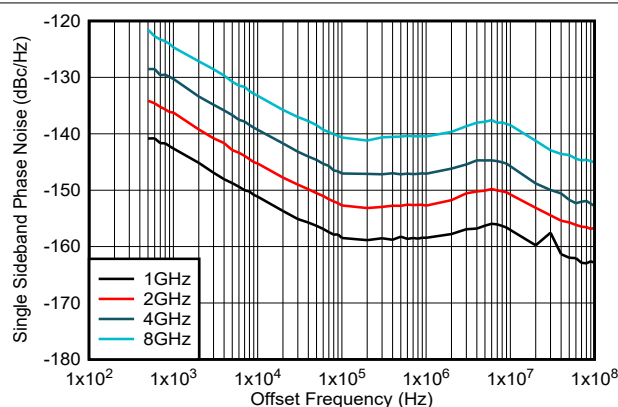
Figure 6-17. Phase Noise in DES2XL Mode, DEM/Dither Off
