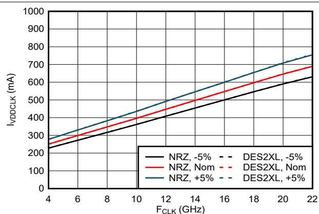
Figure 6-50. I_{VDDCLK} vs Input Clock
