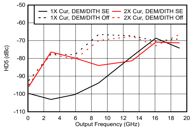
Figure 6-39. HD5 vs Output Frequency in NRZ and RF Modes
