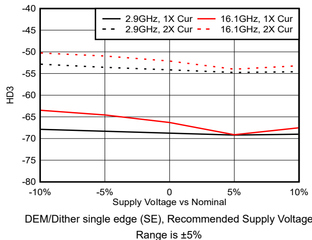
Figure 6-37. HD3 vs Supply Voltage in NRZ and RF Modes
