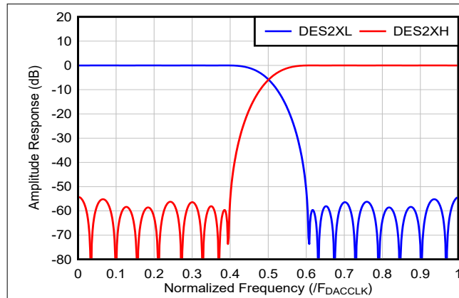
Figure 7-46. DES Interpolator Frequency Response
