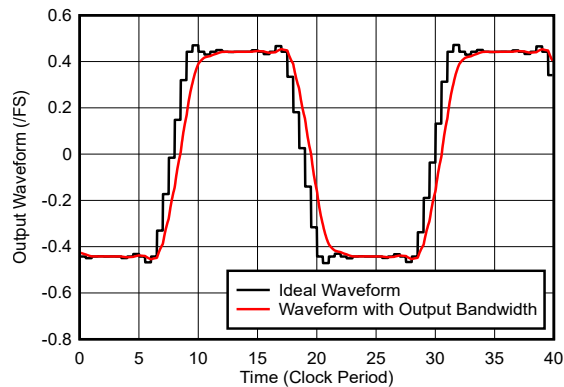
Figure 9-3. Square Wave Output with Recommended Output Bandwidth
