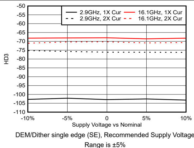
Figure 6-41. HD3 vs Supply Voltage in NRZ and RF Modes
