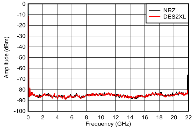
Figure 6-12. Output Spectra at 97MHz, DEM/Dither Off
