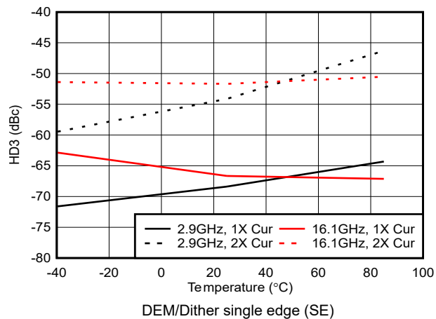
Figure 6-38. HD3 vs Temperature in NRZ and RF Modes
