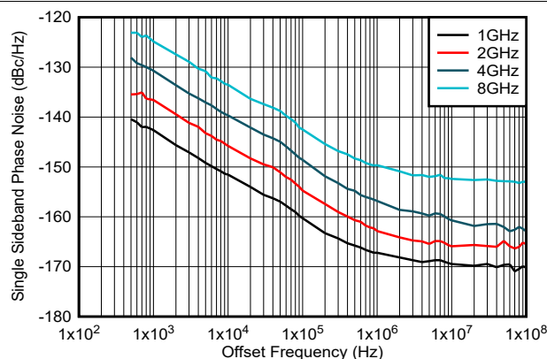
Figure 6-17. Phase Noise in DES2XL Mode, DEM/Dither Off
