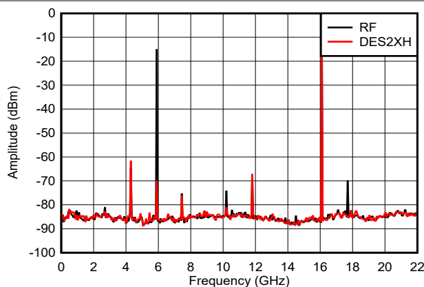
Figure 6-15. Output Spectra at 16097MHz, DEM/Dither On
