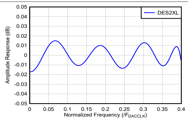
Figure 7-47. DES Interpolator Frequency Response (Passband)
