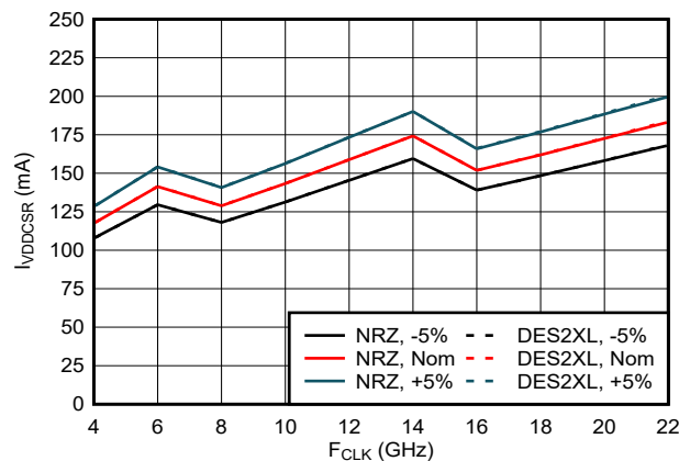
Figure 6-47. I_{VDDCSR} vs Input Clock
