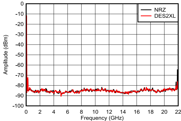
Figure 6-11. Output Spectra at 97MHz, DEM/Dither On
