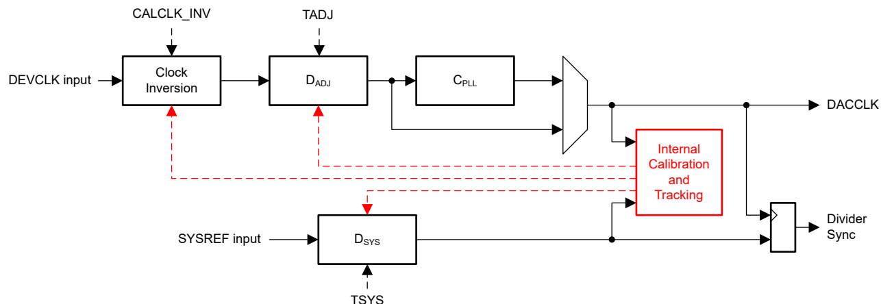
Figure 7-9. Clock and SYSREF Delay Diagram
