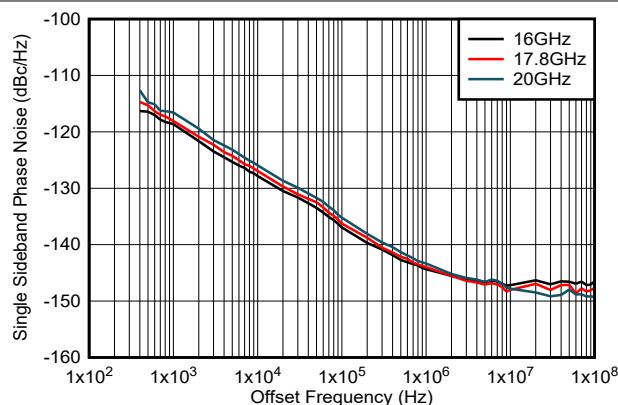
Figure 6-21. Phase Noise in DES2XH Mode, DEM/Dither Off
