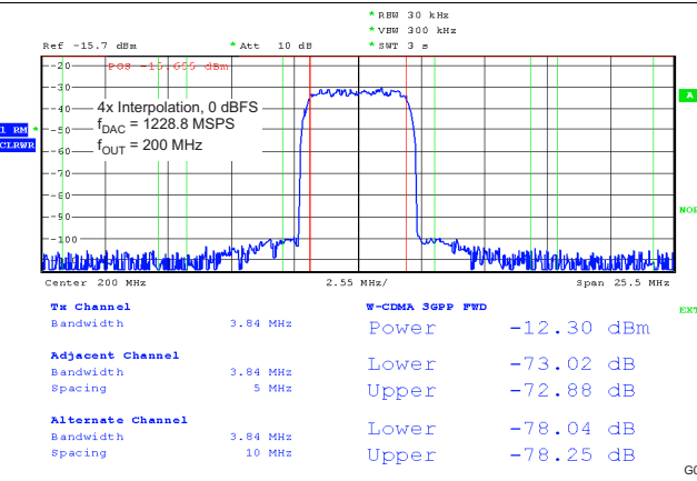
Figure 27. Single Carrier W-CDMA Test Model 1
