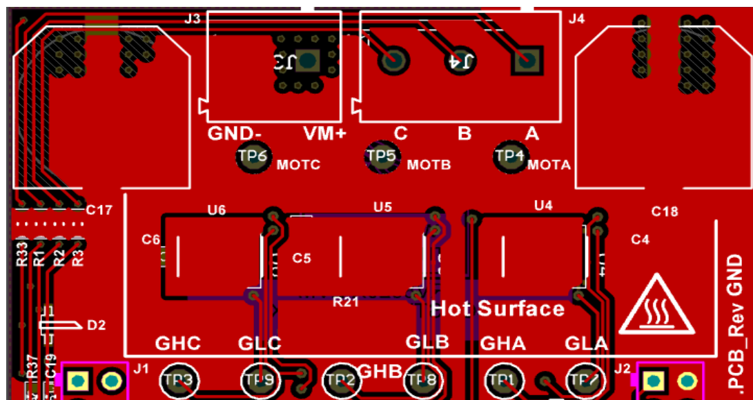
Figure 6-3. Bottom Layer
