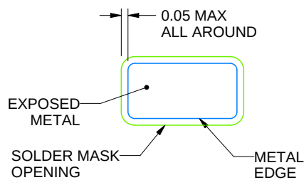
LAND PATTERN EXAMPLE EXPOSED METAL SHOWN SCALE:15X
