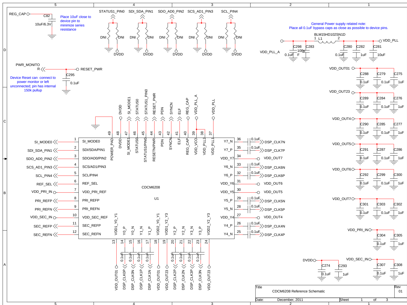
Figure 66. Schematic Page 1
