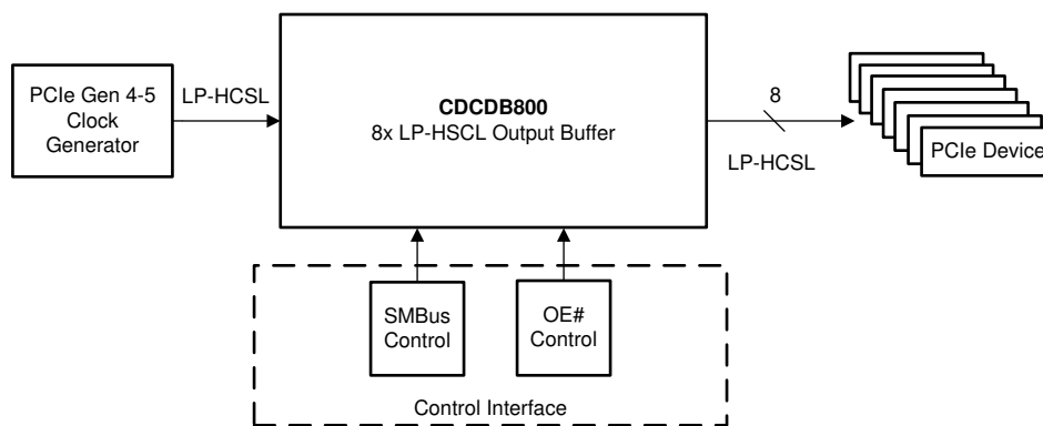
Figure 9-1. Typical Application
