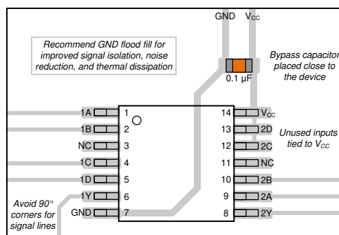
Figure 11-1. Example layout for the CD74HCT20
