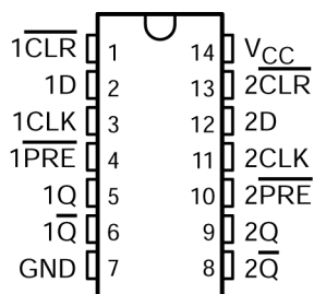
Figure 3-1. D, N, or J Package 14-Pin SOIC, PDIP, or CDIP (Top View)
