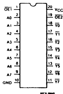
Figure 3-1. CDx4AC540, CDx4ACT540
