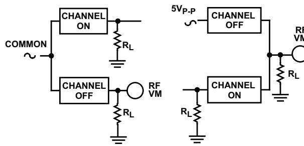
Figure 6-14. Crosstalk Between Any Two Channels (All Types)
