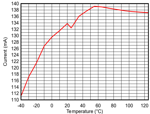
Figure 7-11. TX Current vs Temperature (LE 1M PHY, 2.44GHz, +20dBm), VDDS = 3.3V
