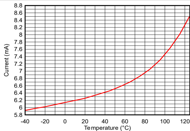
Figure 7-8. RX Current vs Temperature (LE 1M PHY, 2.44GHz), V_{\text{DDS}} = 3.3\text{V}
