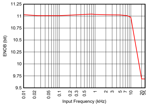
Figure 7-28. ENOB vs Input Frequency (Internal Reference)
